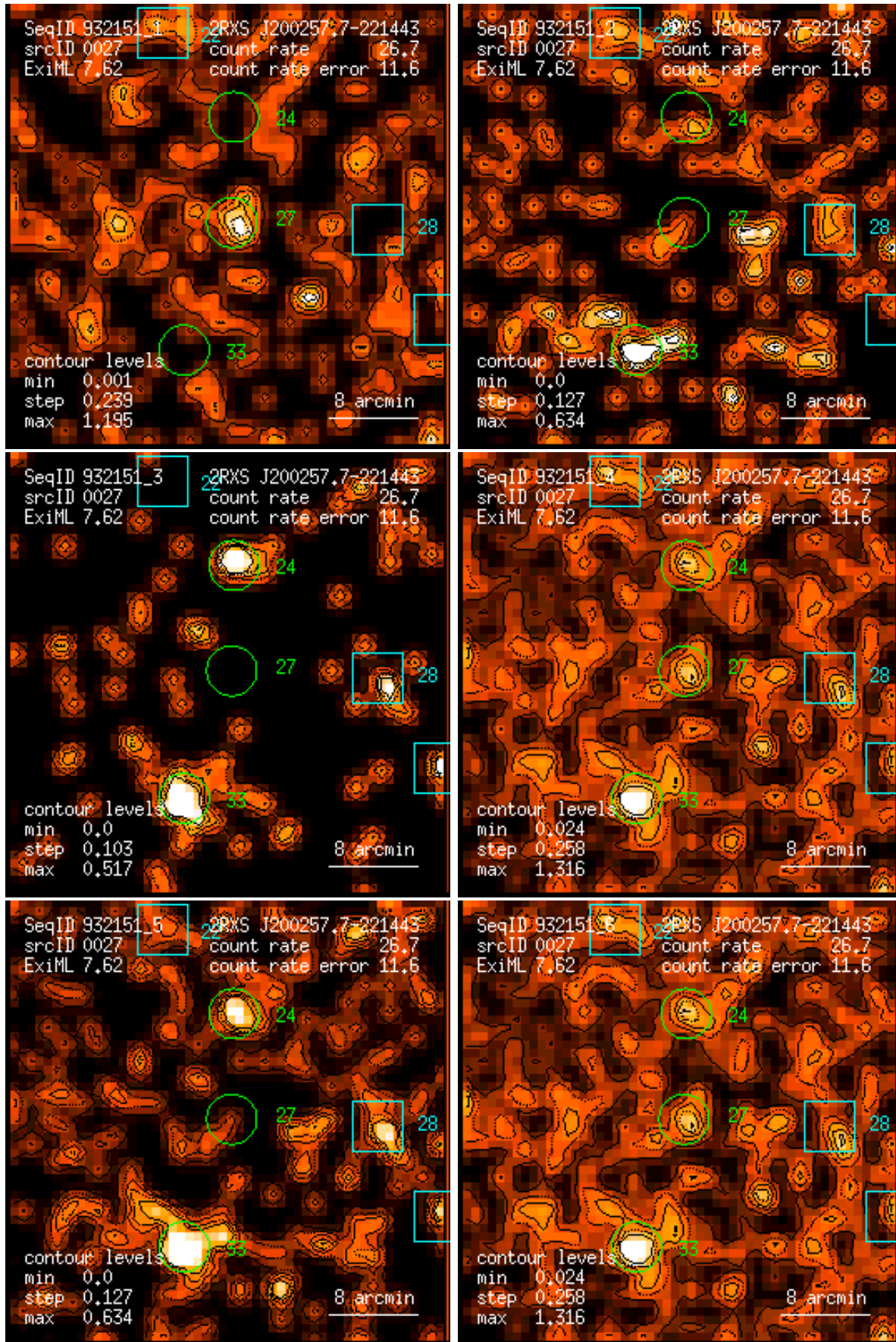
Figure 27: RASS 932151: detection 0027: band rate images, Gaussian filter: (1) PSPC channels 11 – 41, (2) 52 – 90, (3) 91 – 201, (4) 11 – 235, (5) 52 – 201, (6) 11 – 201. Broad band rates in counts/ks. Band rate contour levels in counts/ks/arcmin 2 .
