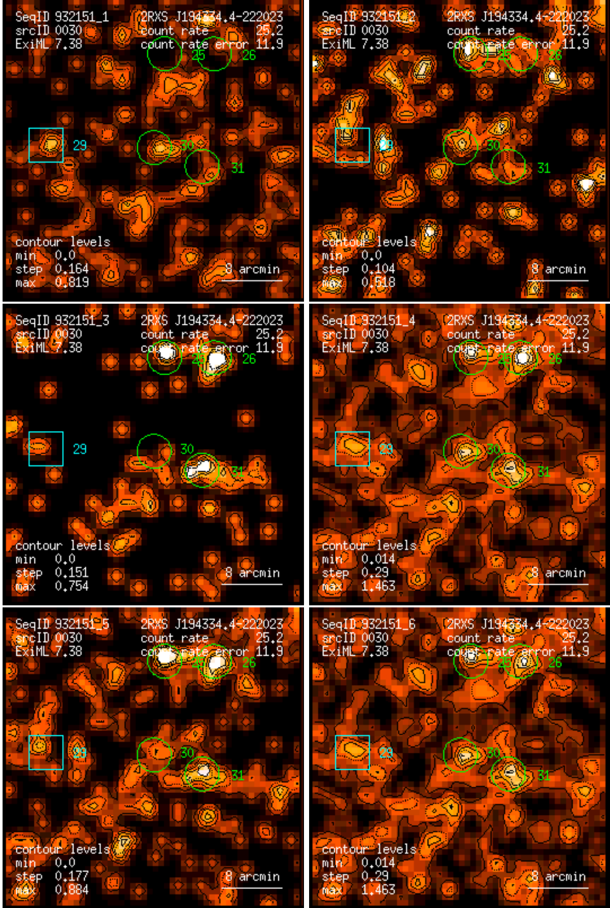
Figure 30: RASS 932151: detection 0030: band rate images, Gaussian filter: (1) PSPC channels 11 – 41, (2) 52 – 90, (3) 91 – 201, (4) 11 – 235, (5) 52 – 201, (6) 11 – 201. Broad band rates in counts/ks. Band rate contour levels in counts/ks/arcmin 2 .
