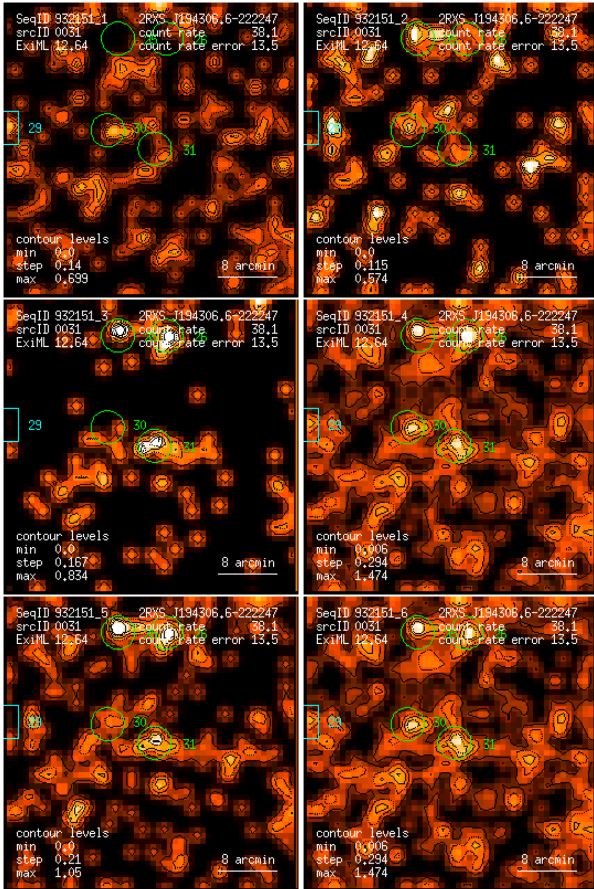
Figure 31: RASS 932151: detection 0031: band rate images, Gaussian filter: (1) PSPC channels 11 – 41, (2) 52 – 90, (3) 91 – 201, (4) 11 – 235, (5) 52 – 201, (6) 11 – 201. Broad band rates in counts/ks. Band rate contour levels in counts/ks/arcmin 2 .
