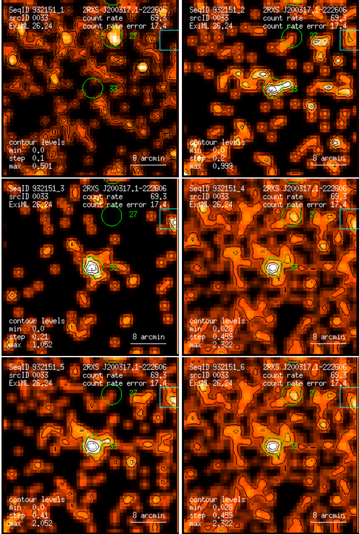
Figure 33: RASS 932151: detection 0033: band rate images, Gaussian filter: (1) PSPC channels 11 – 41, (2) 52 – 90, (3) 91 – 201, (4) 11 – 235, (5) 52 – 201, (6) 11 – 201. Broad band rates in counts/ks. Band rate contour levels in counts/ks/arcmin 2 .
