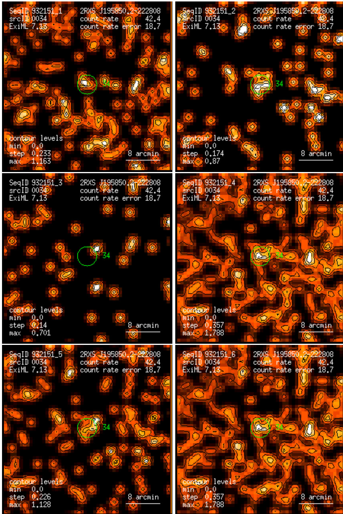
Figure 34: RASS 932151: detection 0034: band rate images, Gaussian filter: (1) PSPC channels 11 – 41, (2) 52 – 90, (3) 91 – 201, (4) 11 – 235, (5) 52 – 201, (6) 11 – 201. Broad band rates in counts/ks. Band rate contour levels in counts/ks/arcmin 2 .
