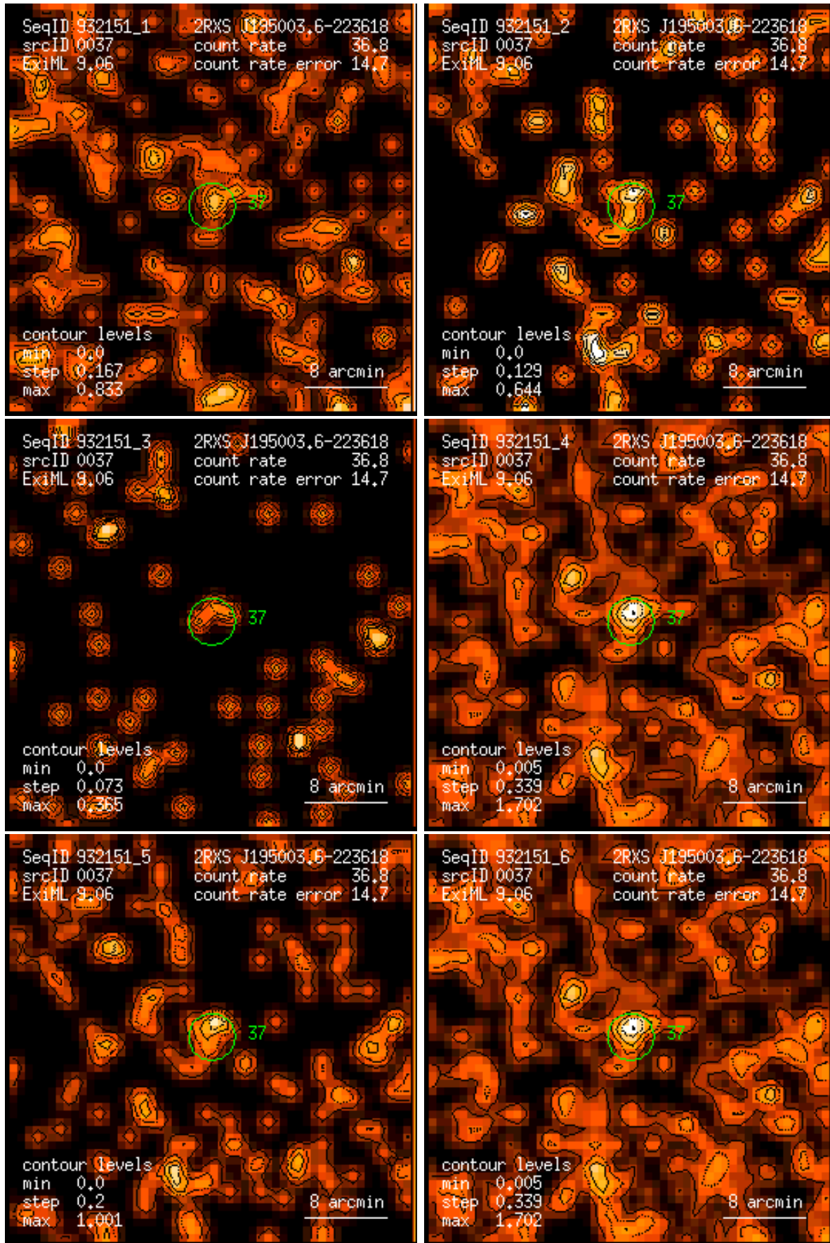
Figure 37: RASS 932151: detection 0037: band rate images, Gaussian filter: (1) PSPC channels 11 – 41, (2) 52 – 90, (3) 91 – 201, (4) 11 – 235, (5) 52 – 201, (6) 11 – 201. Broad band rates in counts/ks. Band rate contour levels in counts/ks/arcmin 2 .
