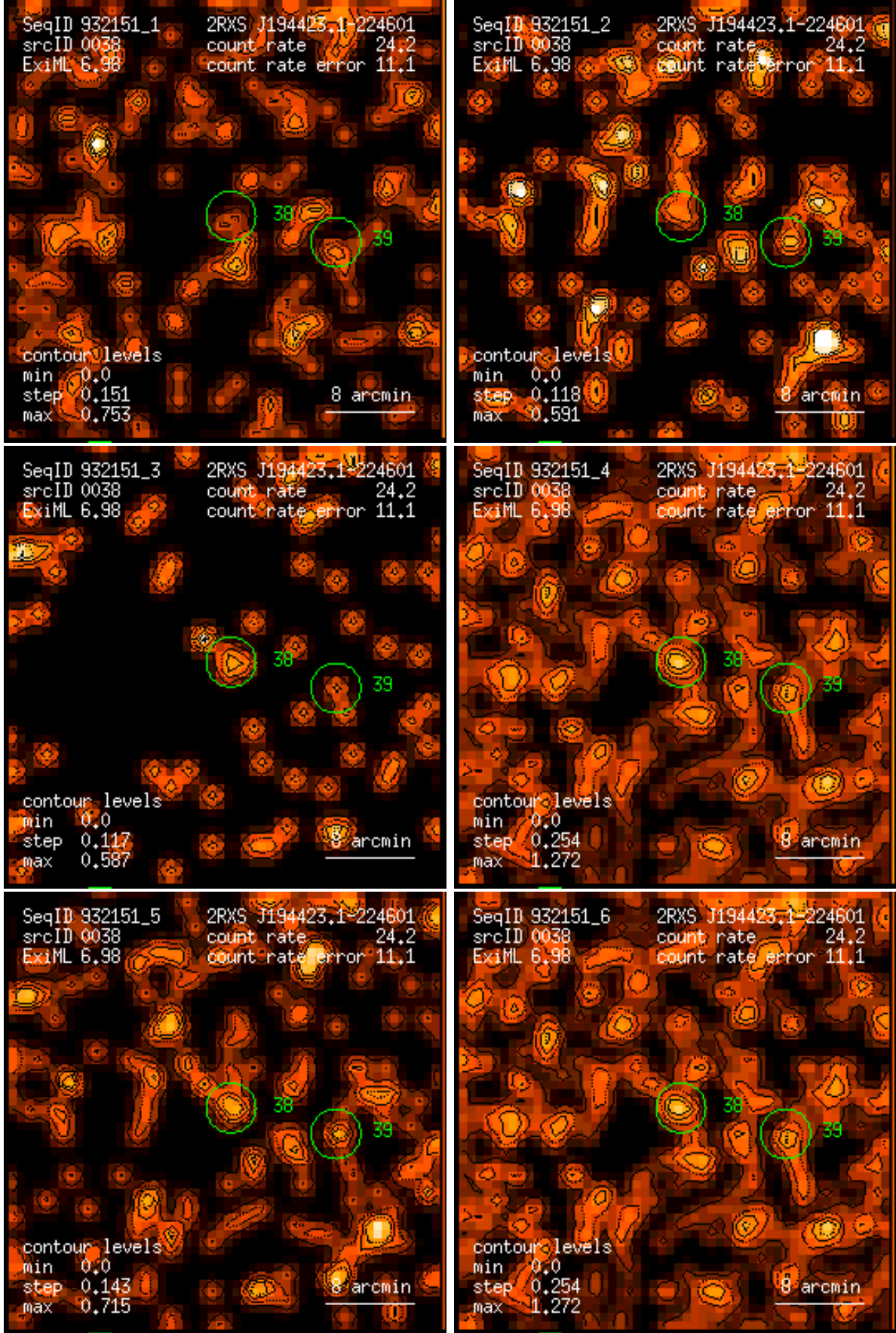
Figure 38: RASS 932151: detection 0038: band rate images, Gaussian filter: (1) PSPC channels 11 – 41, (2) 52 – 90, (3) 91 – 201, (4) 11 – 235, (5) 52 – 201, (6) 11 – 201. Broad band rates in counts/ks. Band rate contour levels in counts/ks/arcmin 2 .
