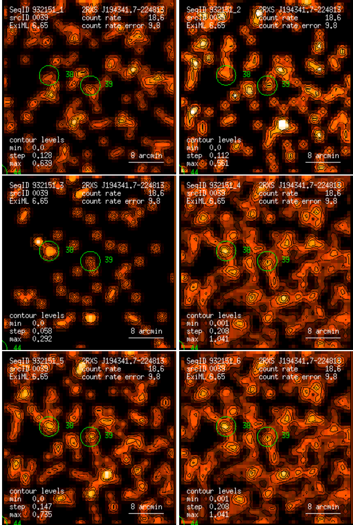
Figure 39: RASS 932151: detection 0039: band rate images, Gaussian filter: (1) PSPC channels 11 – 41, (2) 52 – 90, (3) 91 – 201, (4) 11 – 235, (5) 52 – 201, (6) 11 – 201. Broad band rates in counts/ks. Band rate contour levels in counts/ks/arcmin 2 .
