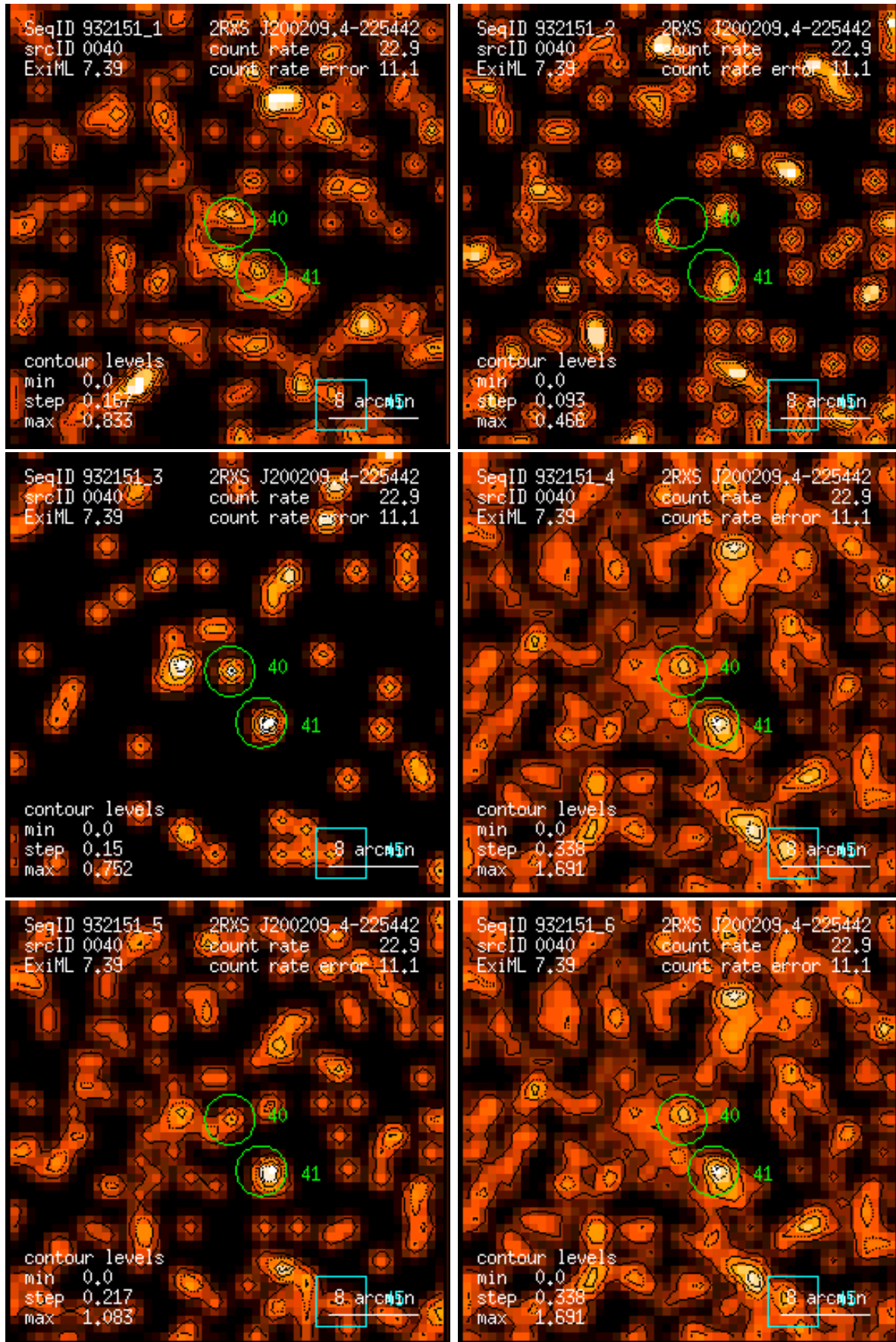
Figure 40: RASS 932151: detection 0040: band rate images, Gaussian filter: (1) PSPC channels 11 – 41, (2) 52 – 90, (3) 91 – 201, (4) 11 – 235, (5) 52 – 201, (6) 11 – 201. Broad band rates in counts/ks. Band rate contour levels in counts/ks/arcmin 2 .
