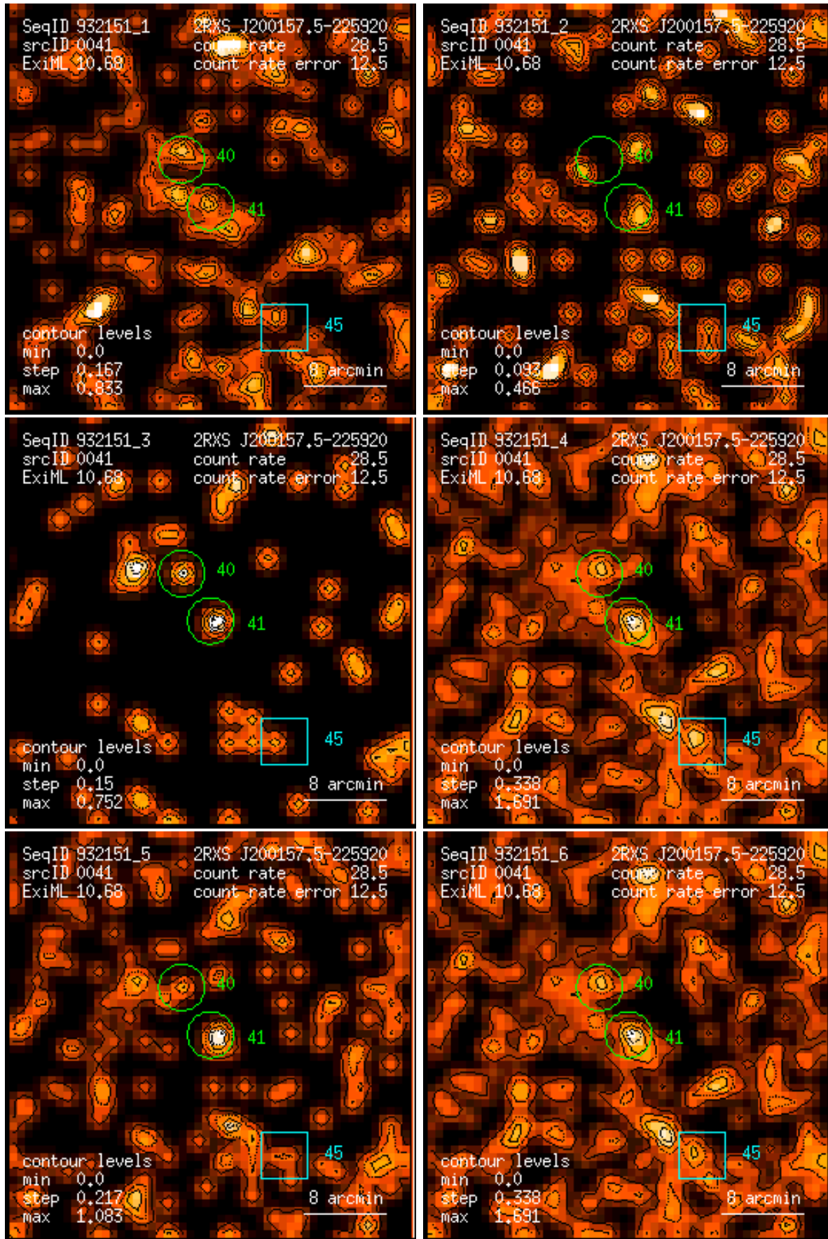
Figure 41: RASS 932151: detection 0041: band rate images, Gaussian filter: (1) PSPC channels 11 – 41, (2) 52 – 90, (3) 91 – 201, (4) 11 – 235, (5) 52 – 201, (6) 11 – 201. Broad band rates in counts/ks. Band rate contour levels in counts/ks/arcmin 2 .
