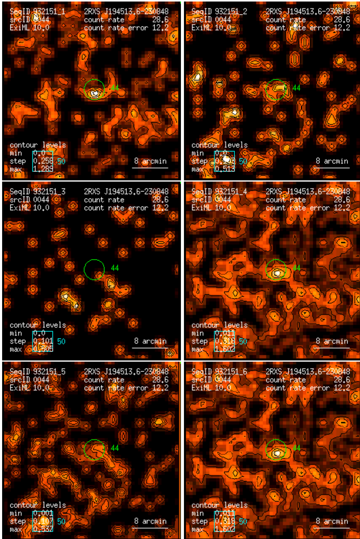
Figure 44: RASS 932151: detection 0044: band rate images, Gaussian filter: (1) PSPC channels 11 – 41, (2) 52 – 90, (3) 91 – 201, (4) 11 – 235, (5) 52 – 201, (6) 11 – 201. Broad band rates in counts/ks. Band rate contour levels in counts/ks/arcmin 2 .
