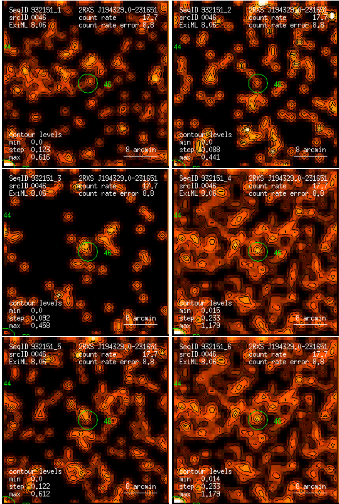
Figure 46: RASS 932151: detection 0046: band rate images, Gaussian filter: (1) PSPC channels 11 – 41, (2) 52 – 90, (3) 91 – 201, (4) 11 – 235, (5) 52 – 201, (6) 11 – 201. Broad band rates in counts/ks. Band rate contour levels in counts/ks/arcmin 2 .
