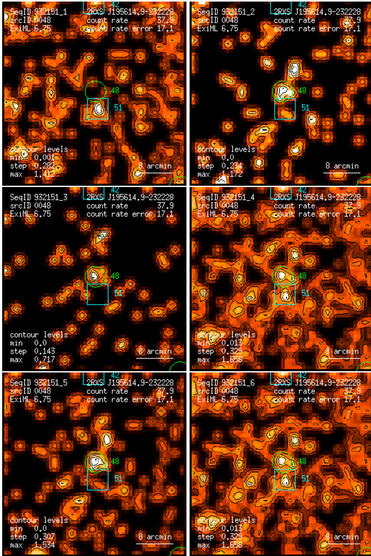
Figure 48: RASS 932151: detection 0048: band rate images, Gaussian filter: (1) PSPC channels 11 – 41, (2) 52 – 90, (3) 91 – 201, (4) 11 – 235, (5) 52 – 201, (6) 11 – 201. Broad band rates in counts/ks. Band rate contour levels in counts/ks/arcmin 2 .
