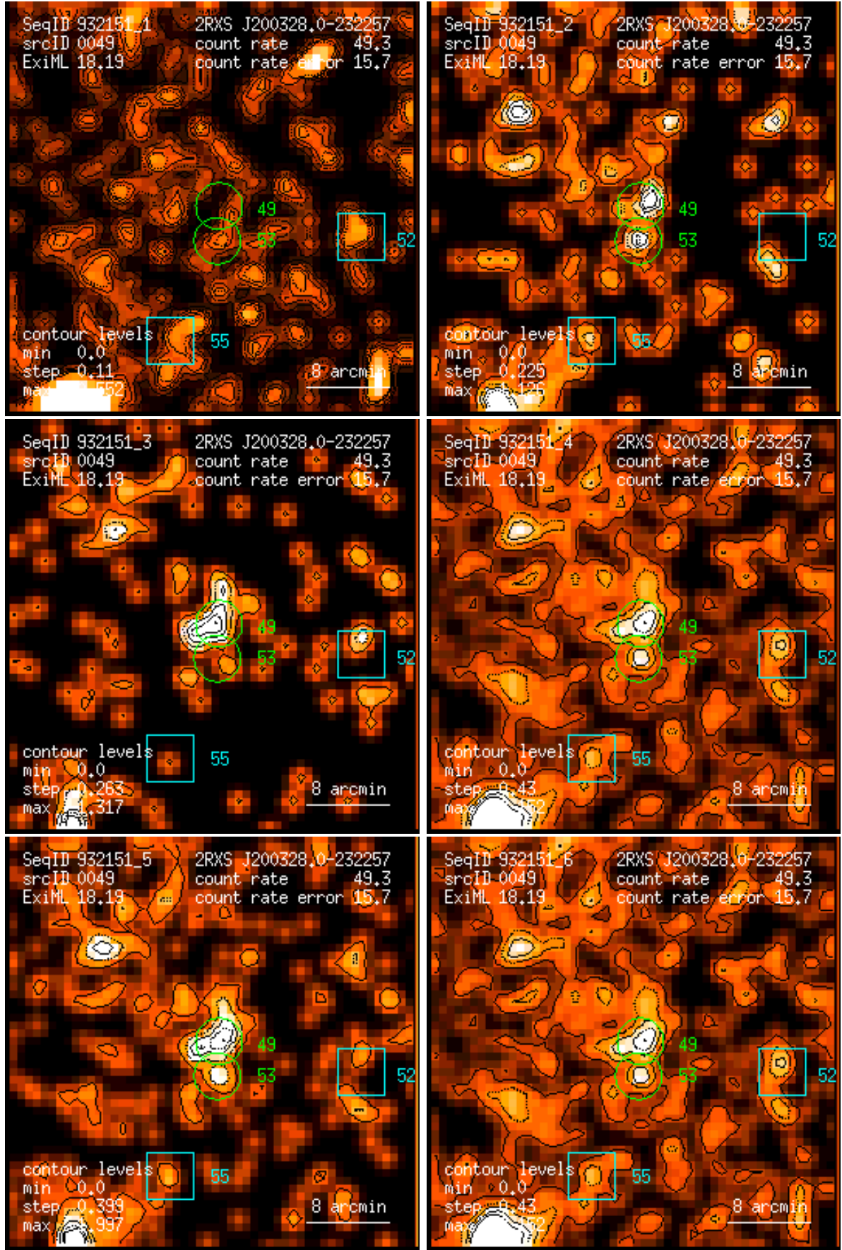
Figure 49: RASS 932151: detection 0049: band rate images, Gaussian filter: (1) PSPC channels 11 – 41, (2) 52 – 90, (3) 91 – 201, (4) 11 – 235, (5) 52 – 201, (6) 11 – 201. Broad band rates in counts/ks. Band rate contour levels in counts/ks/arcmin 2 .
