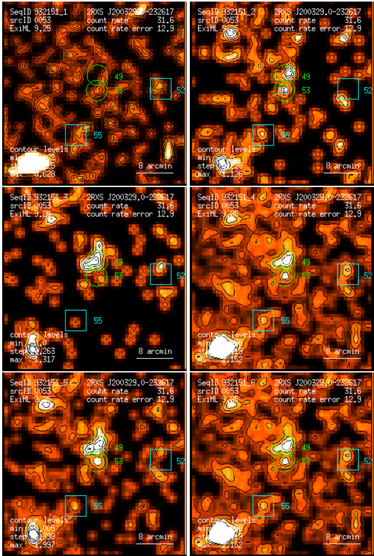
Figure 53: RASS 932151: detection 0053: band rate images, Gaussian filter: (1) PSPC channels 11 – 41, (2) 52 – 90, (3) 91 – 201, (4) 11 – 235, (5) 52 – 201, (6) 11 – 201. Broad band rates in counts/ks. Band rate contour levels in counts/ks/arcmin 2 .
