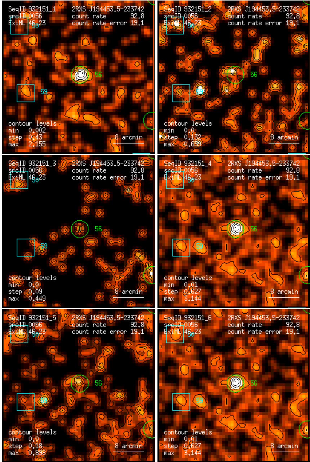
Figure 56: RASS 932151: detection 0056: band rate images, Gaussian filter: (1) PSPC channels 11 – 41, (2) 52 – 90, (3) 91 – 201, (4) 11 – 235, (5) 52 – 201, (6) 11 – 201. Broad band rates in counts/ks. Band rate contour levels in counts/ks/arcmin 2 .
