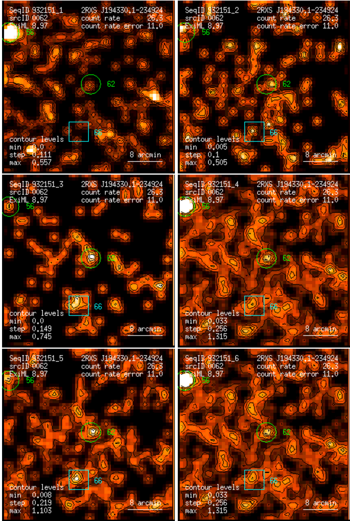
Figure 62: RASS 932151: detection 0062: band rate images, Gaussian filter: (1) PSPC channels 11 – 41, (2) 52 – 90, (3) 91 – 201, (4) 11 – 235, (5) 52 – 201, (6) 11 – 201. Broad band rates in counts/ks. Band rate contour levels in counts/ks/arcmin 2 .
