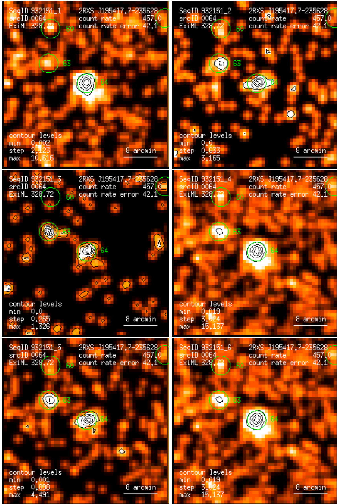
Figure 64: RASS 932151: detection 0064: band rate images, Gaussian filter: (1) PSPC channels 11 – 41, (2) 52 – 90, (3) 91 – 201, (4) 11 – 235, (5) 52 – 201, (6) 11 – 201. Broad band rates in counts/ks. Band rate contour levels in counts/ks/arcmin 2 .
