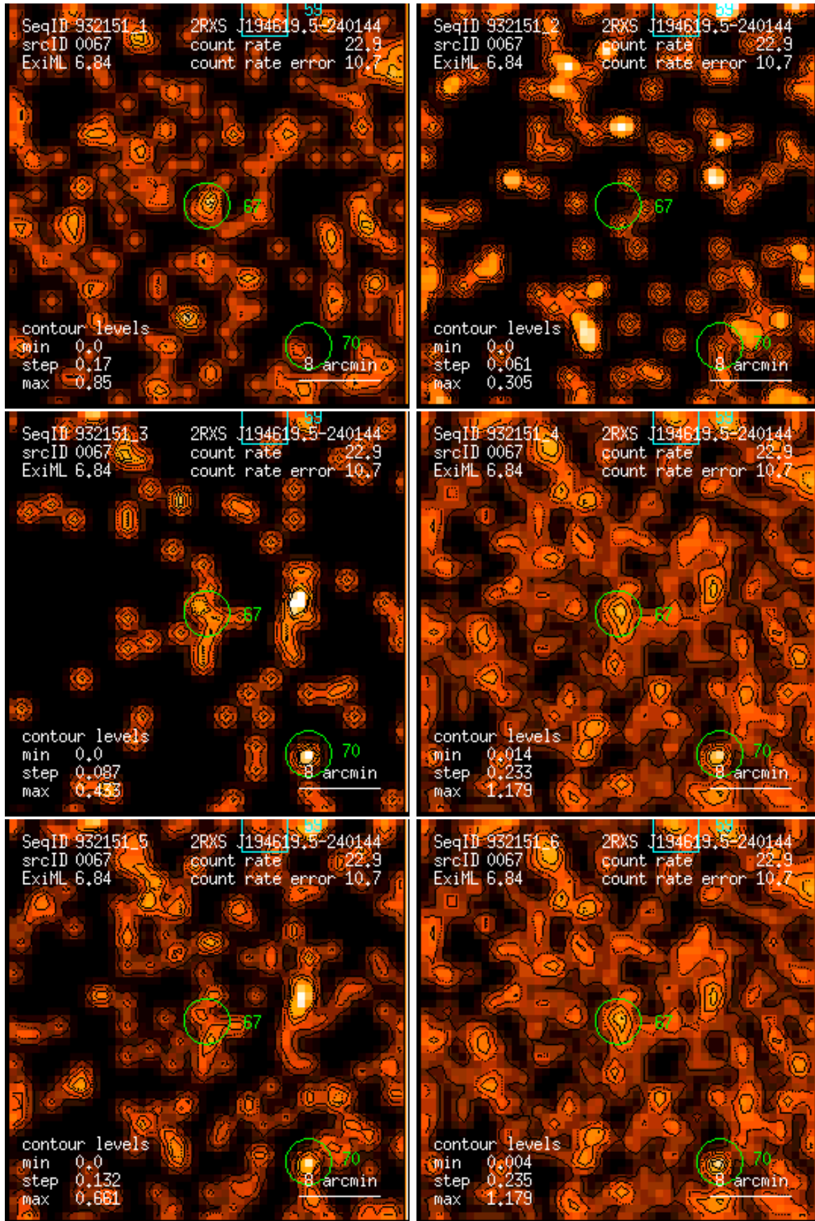
Figure 67: RASS 932151: detection 0067: band rate images, Gaussian filter: (1) PSPC channels 11 – 41, (2) 52 – 90, (3) 91 – 201, (4) 11 – 235, (5) 52 – 201, (6) 11 – 201. Broad band rates in counts/ks. Band rate contour levels in counts/ks/arcmin 2 .
