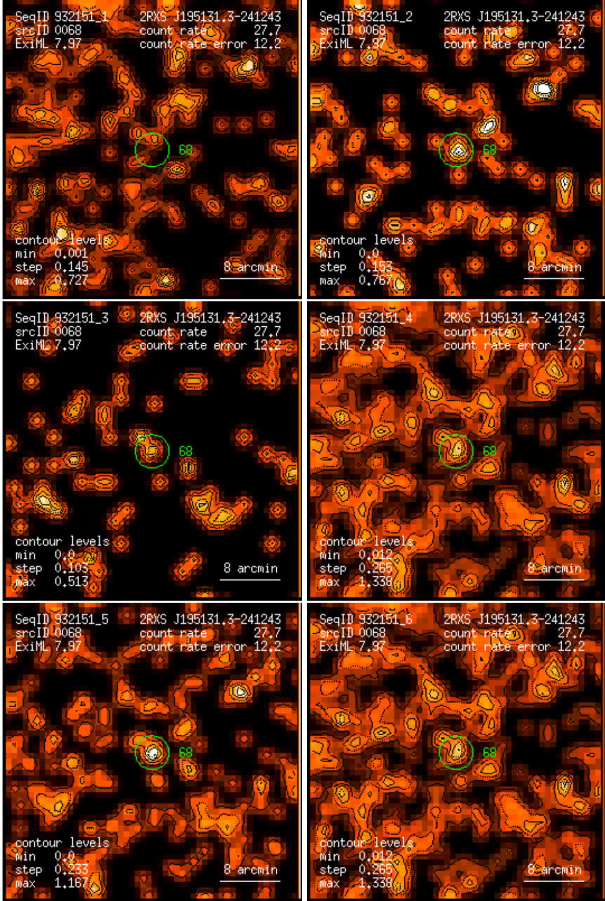
Figure 68: RASS 932151: detection 0068: band rate images, Gaussian filter: (1) PSPC channels 11 – 41, (2) 52 – 90, (3) 91 – 201, (4) 11 – 235, (5) 52 – 201, (6) 11 – 201. Broad band rates in counts/ks. Band rate contour levels in counts/ks/arcmin 2 .
