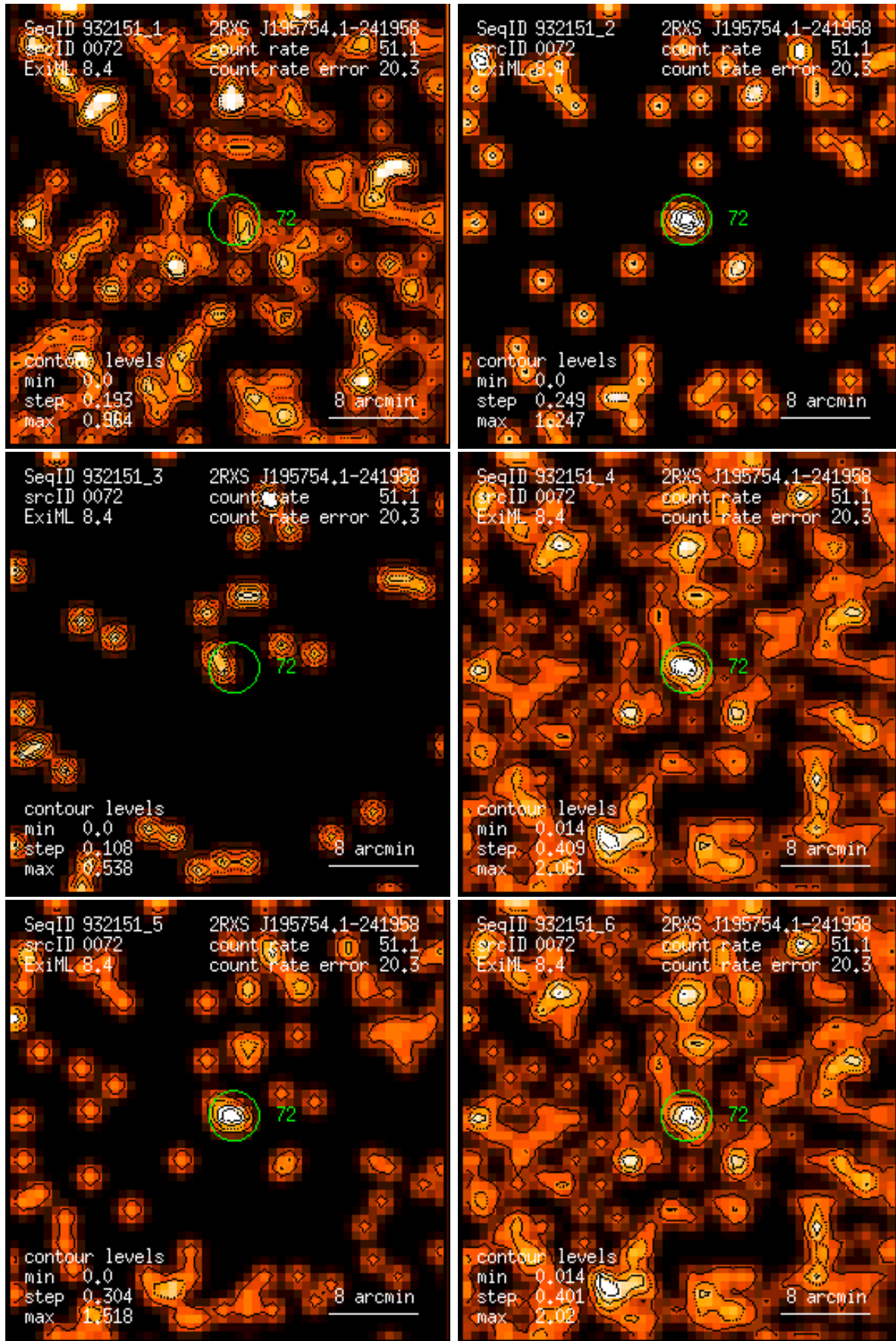
Figure 72: RASS 932151: detection 0072: band rate images, Gaussian filter: (1) PSPC channels 11 – 41, (2) 52 – 90, (3) 91 – 201, (4) 11 – 235, (5) 52 – 201, (6) 11 – 201. Broad band rates in counts/ks. Band rate contour levels in counts/ks/arcmin 2 .
