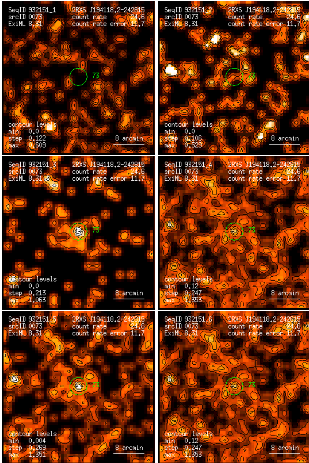
Figure 73: RASS 932151: detection 0073: band rate images, Gaussian filter: (1) PSPC channels 11 – 41, (2) 52 – 90, (3) 91 – 201, (4) 11 – 235, (5) 52 – 201, (6) 11 – 201. Broad band rates in counts/ks. Band rate contour levels in counts/ks/arcmin 2 .
