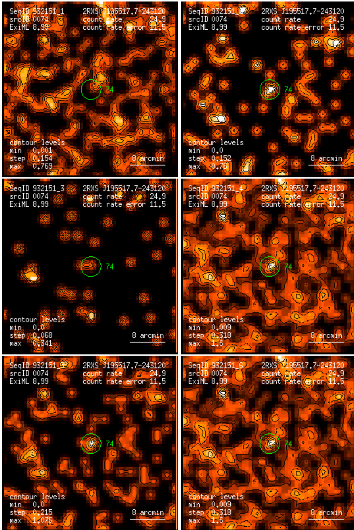
Figure 74: RASS 932151: detection 0074: band rate images, Gaussian filter: (1) PSPC channels 11 – 41, (2) 52 – 90, (3) 91 – 201, (4) 11 – 235, (5) 52 – 201, (6) 11 – 201. Broad band rates in counts/ks. Band rate contour levels in counts/ks/arcmin 2 .
