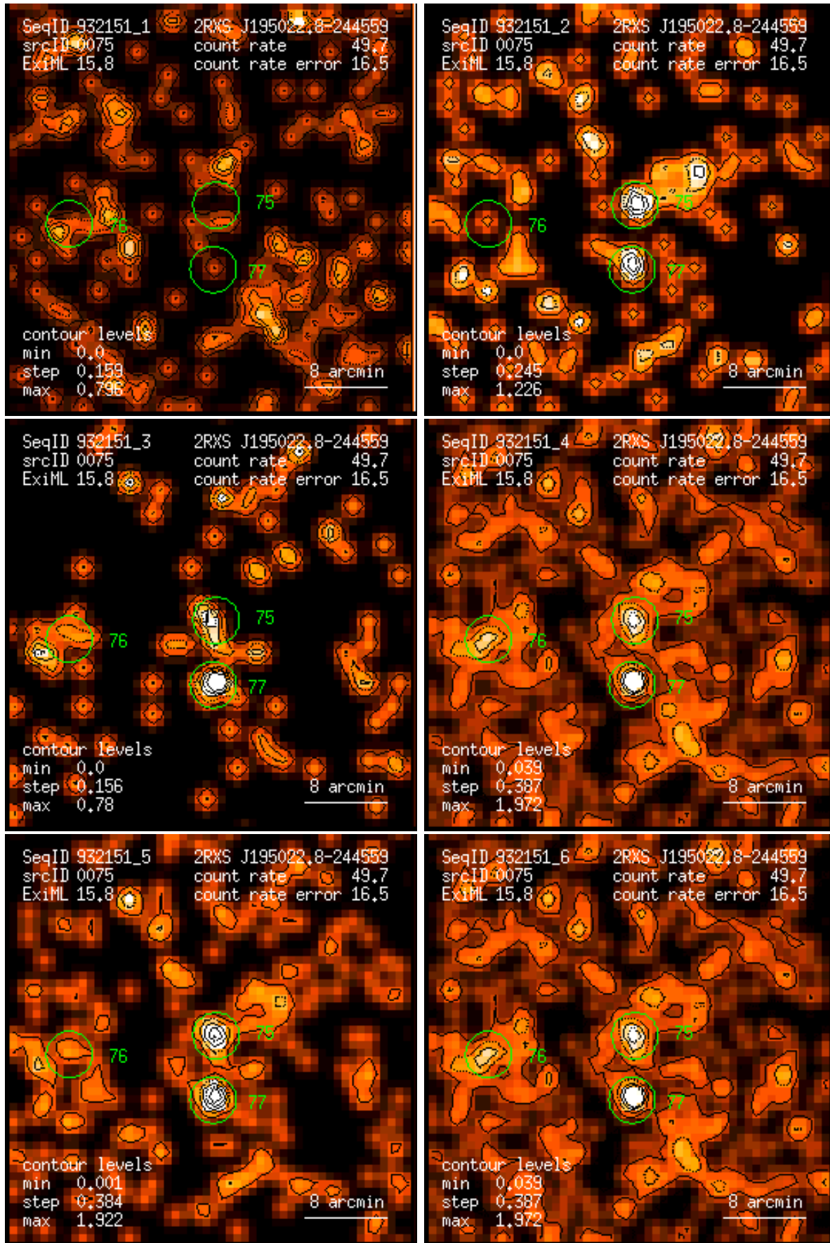
Figure 75: RASS 932151: detection 0075: band rate images, Gaussian filter: (1) PSPC channels 11 – 41, (2) 52 – 90, (3) 91 – 201, (4) 11 – 235, (5) 52 – 201, (6) 11 – 201. Broad band rates in counts/ks. Band rate contour levels in counts/ks/arcmin 2 .
