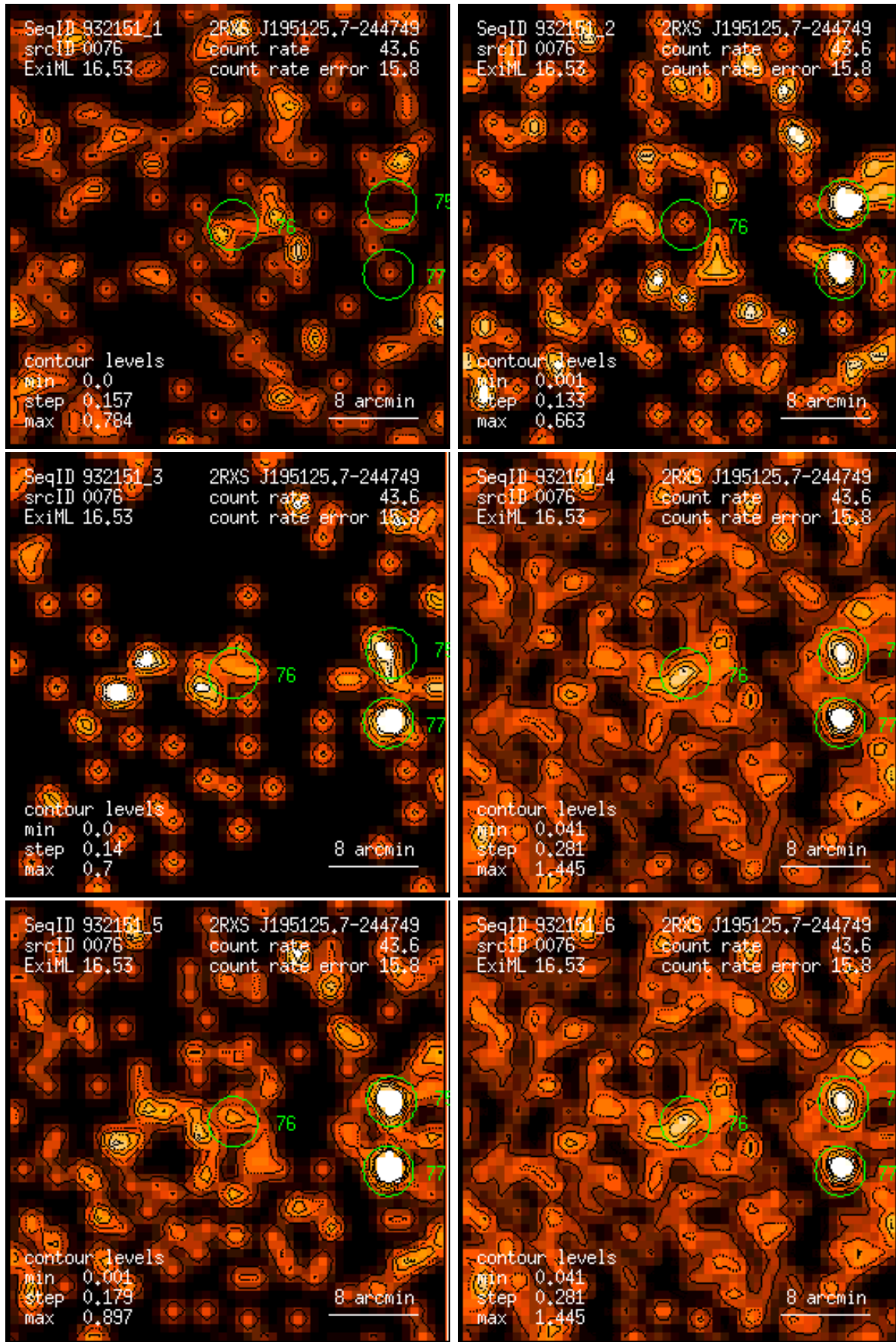
Figure 76: RASS 932151: detection 0076: band rate images, Gaussian filter: (1) PSPC channels 11 – 41, (2) 52 – 90, (3) 91 – 201, (4) 11 – 235, (5) 52 – 201, (6) 11 – 201. Broad band rates in counts/ks. Band rate contour levels in counts/ks/arcmin 2 .
