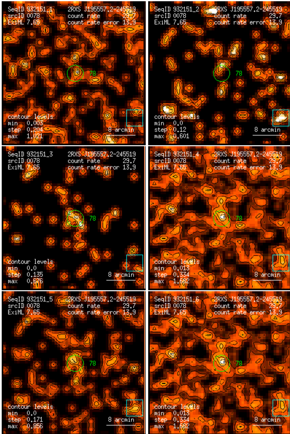
Figure 78: RASS 932151: detection 0078: band rate images, Gaussian filter: (1) PSPC channels 11 – 41, (2) 52 – 90, (3) 91 – 201, (4) 11 – 235, (5) 52 – 201, (6) 11 – 201. Broad band rates in counts/ks. Band rate contour levels in counts/ks/arcmin 2 .
