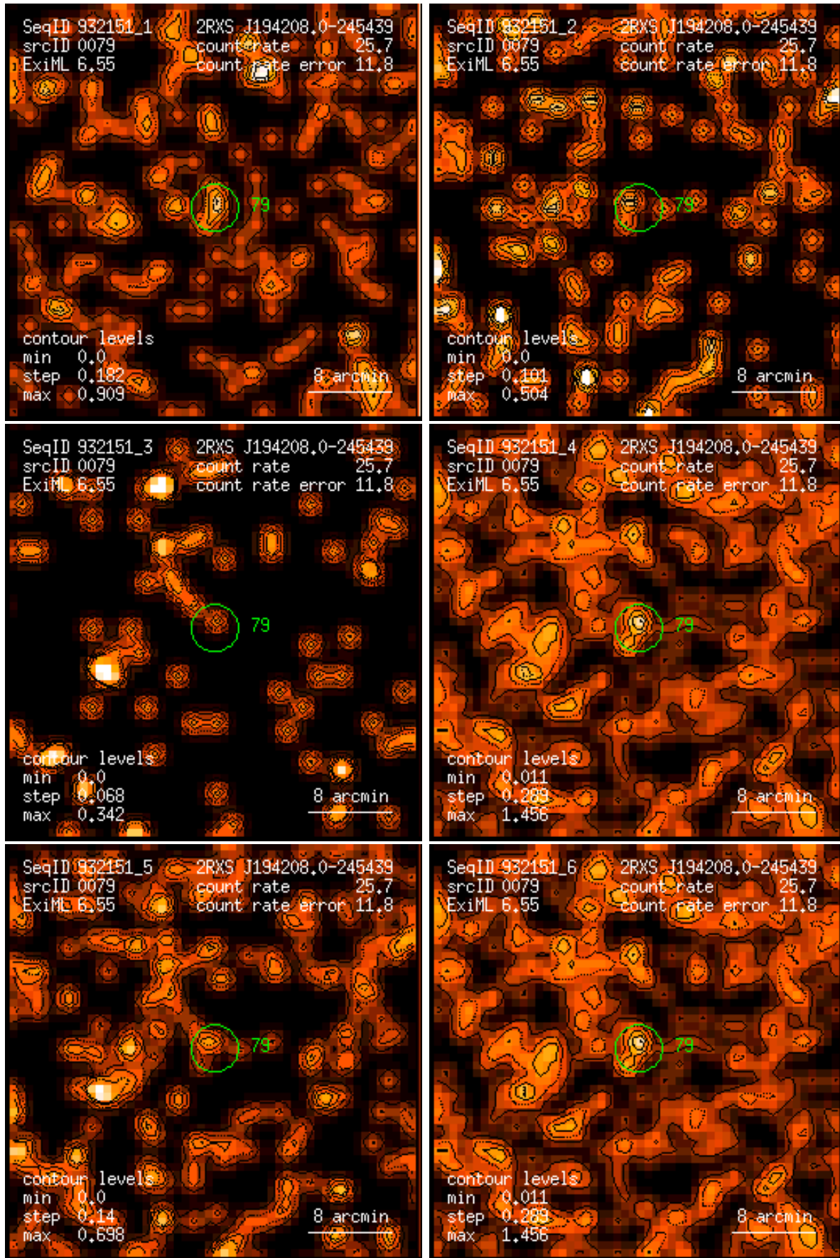
Figure 79: RASS 932151: detection 0079: band rate images, Gaussian filter: (1) PSPC channels 11 – 41, (2) 52 – 90, (3) 91 – 201, (4) 11 – 235, (5) 52 – 201, (6) 11 – 201. Broad band rates in counts/ks. Band rate contour levels in counts/ks/arcmin 2 .
