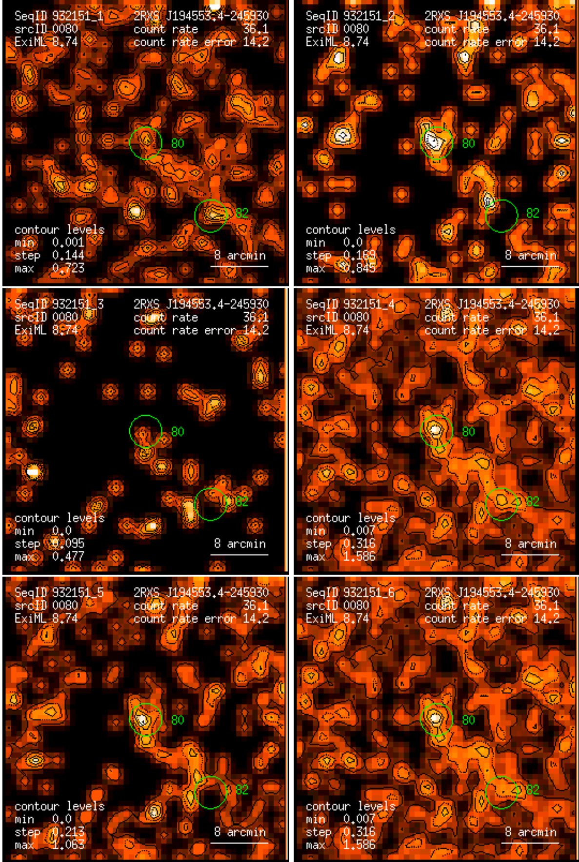
Figure 80: RASS 932151: detection 0080: band rate images, Gaussian filter: (1) PSPC channels 11 – 41, (2) 52 – 90, (3) 91 – 201, (4) 11 – 235, (5) 52 – 201, (6) 11 – 201. Broad band rates in counts/ks. Band rate contour levels in counts/ks/arcmin 2 .
