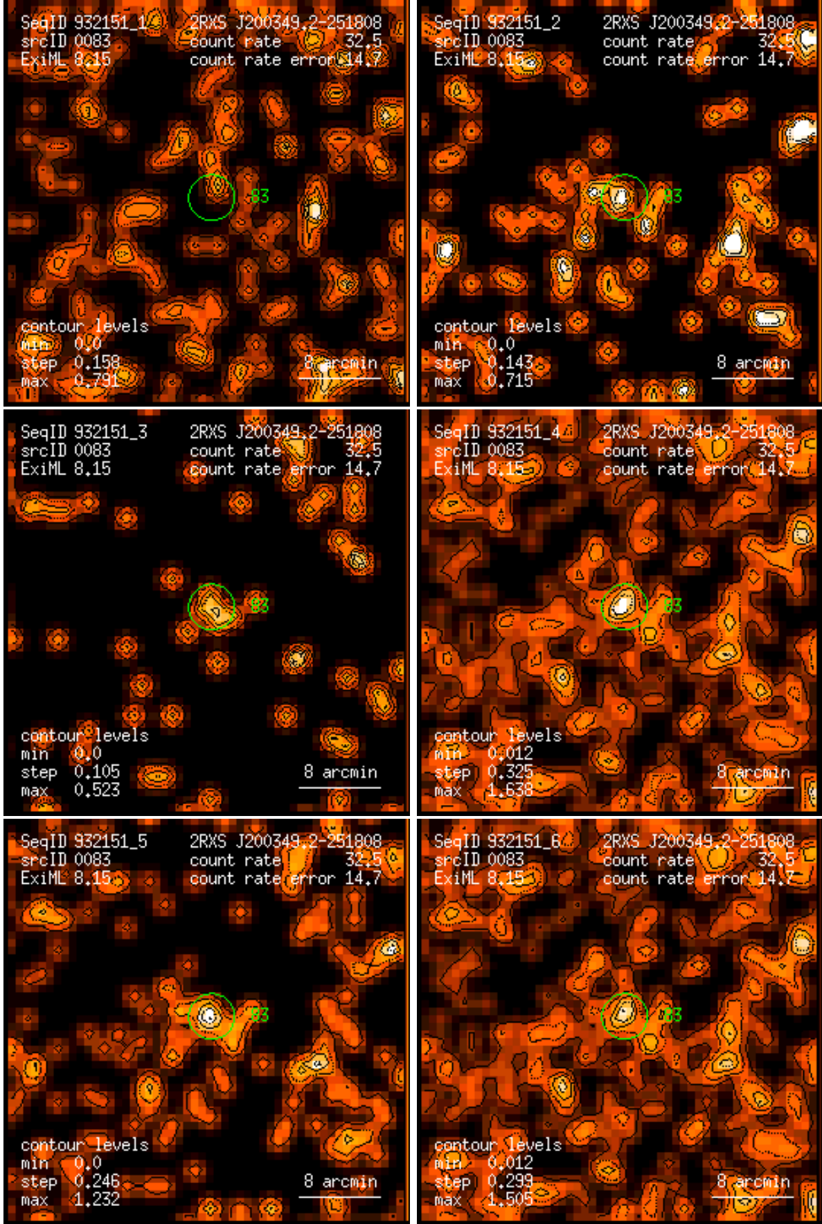
Figure 83: RASS 932151: detection 0083: band rate images, Gaussian filter: (1) PSPC channels 11 – 41, (2) 52 – 90, (3) 91 – 201, (4) 11 – 235, (5) 52 – 201, (6) 11 – 201. Broad band rates in counts/ks. Band rate contour levels in counts/ks/arcmin 2 .
