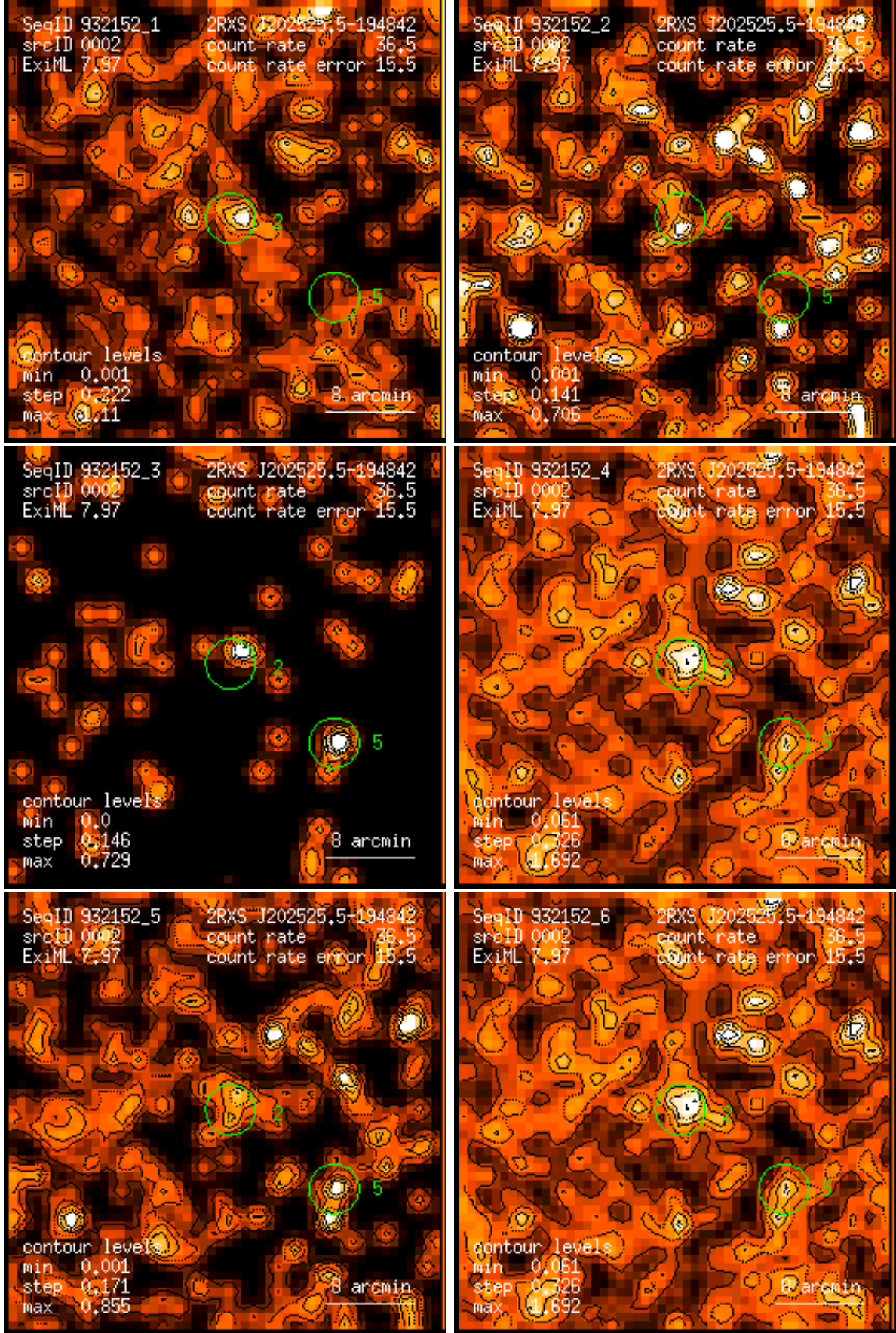
Figure 2: RASS 932152: detection 0002: band rate images, Gaussian filter: (1) PSPC channels 11 – 41, (2) 52 – 90, (3) 91 – 201, (4) 11 – 235, (5) 52 – 201, (6) 11 – 201. Broad band rates in counts/ks. Band rate contour levels in counts/ks/arcmin 2 .
