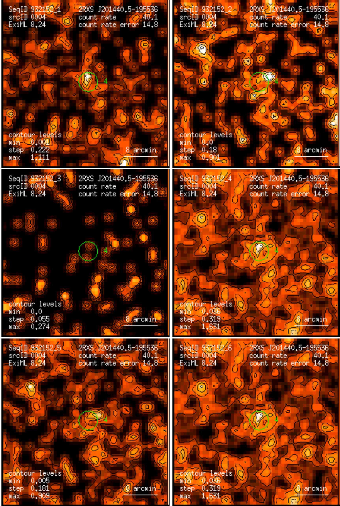
Figure 4: RASS 932152: detection 0004: band rate images, Gaussian filter: (1) PSPC channels 11 – 41, (2) 52 – 90, (3) 91 – 201, (4) 11 – 235, (5) 52 – 201, (6) 11 – 201. Broad band rates in counts/ks. Band rate contour levels in counts/ks/arcmin 2 .
