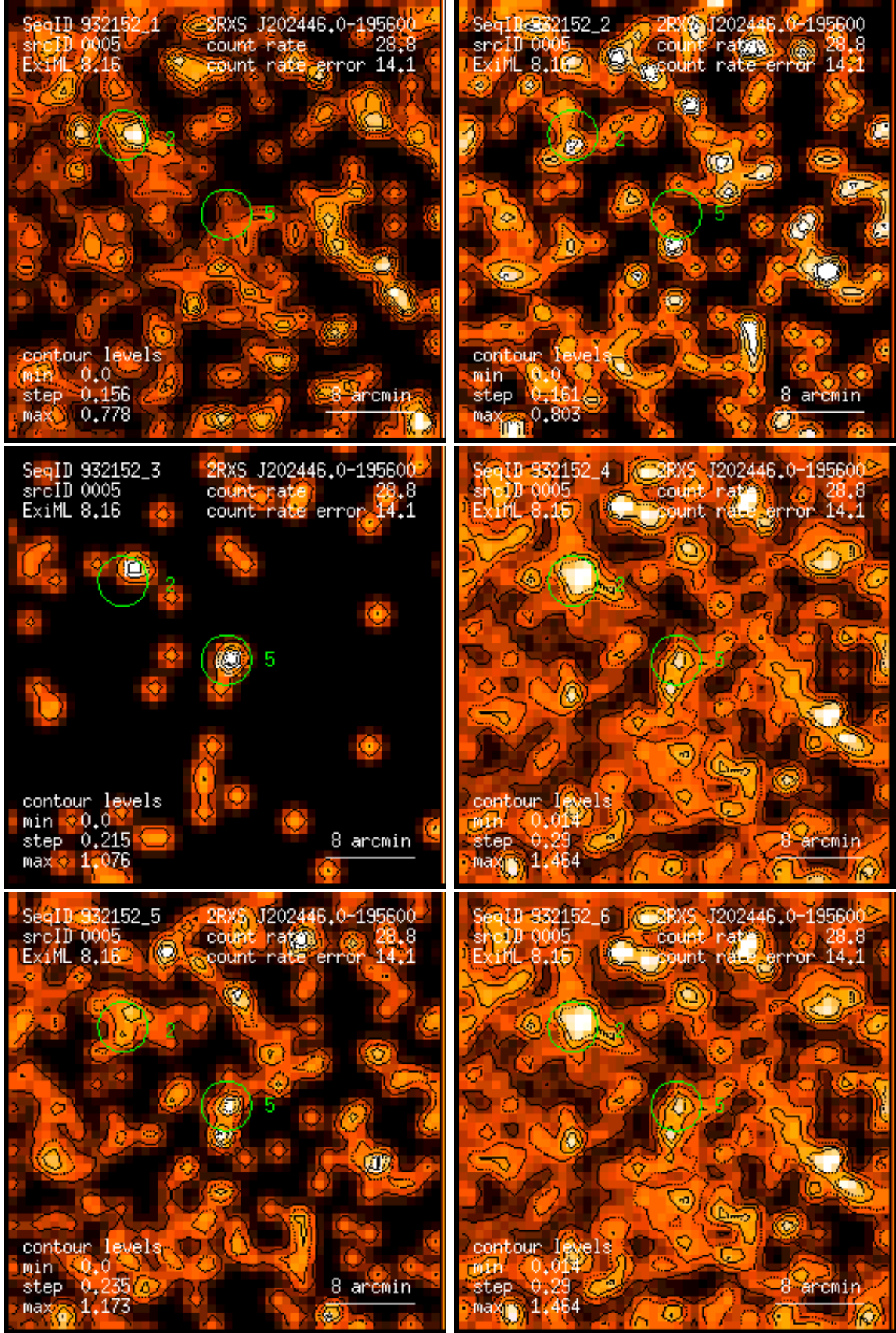
Figure 5: RASS 932152: detection 0005: band rate images, Gaussian filter: (1) PSPC channels 11 – 41, (2) 52 – 90, (3) 91 – 201, (4) 11 – 235, (5) 52 – 201, (6) 11 – 201. Broad band rates in counts/ks. Band rate contour levels in counts/ks/arcmin 2 .
