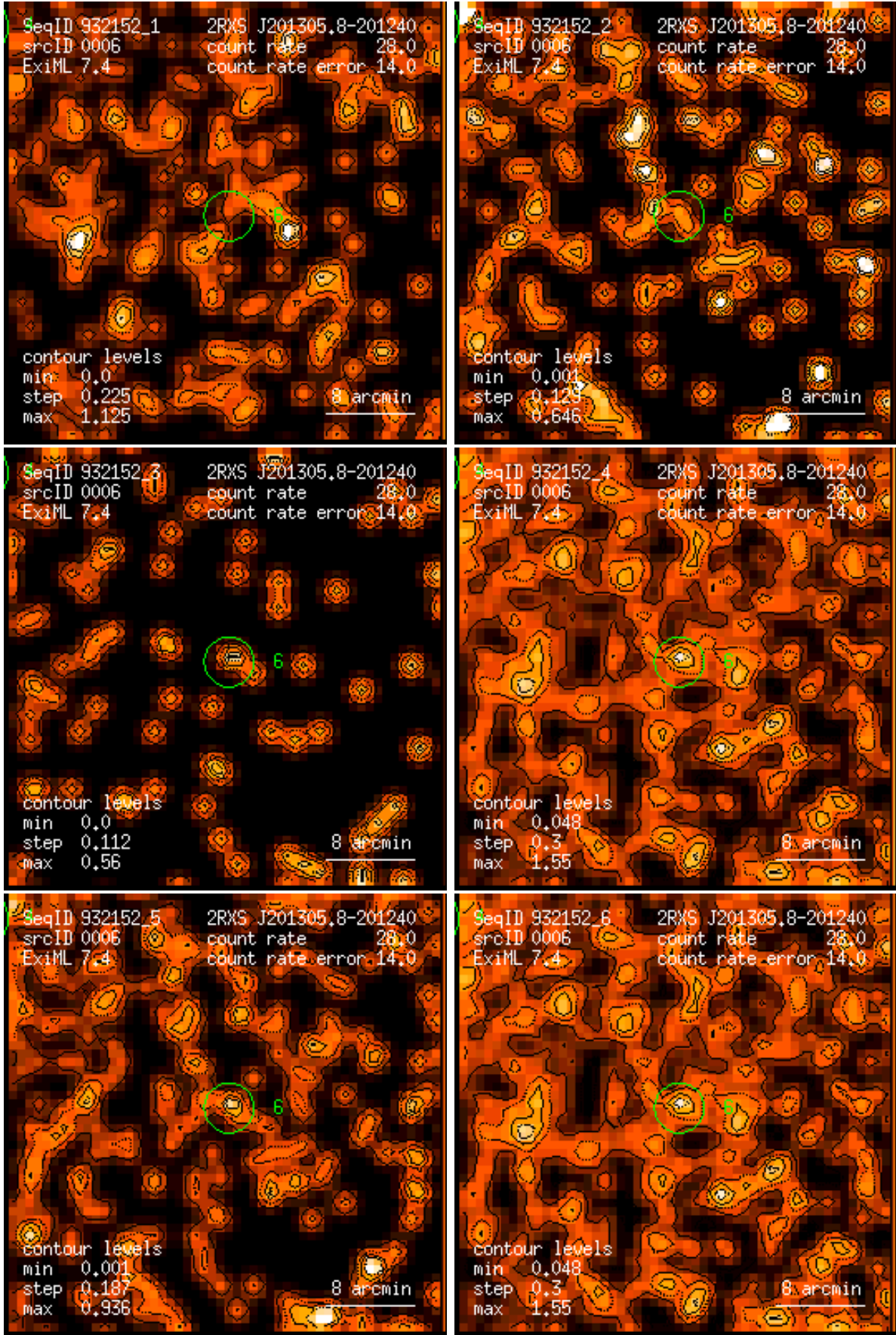
Figure 6: RASS 932152: detection 0006: band rate images, Gaussian filter: (1) PSPC channels 11 – 41, (2) 52 – 90, (3) 91 – 201, (4) 11 – 235, (5) 52 – 201, (6) 11 – 201. Broad band rates in counts/ks. Band rate contour levels in counts/ks/arcmin 2 .
