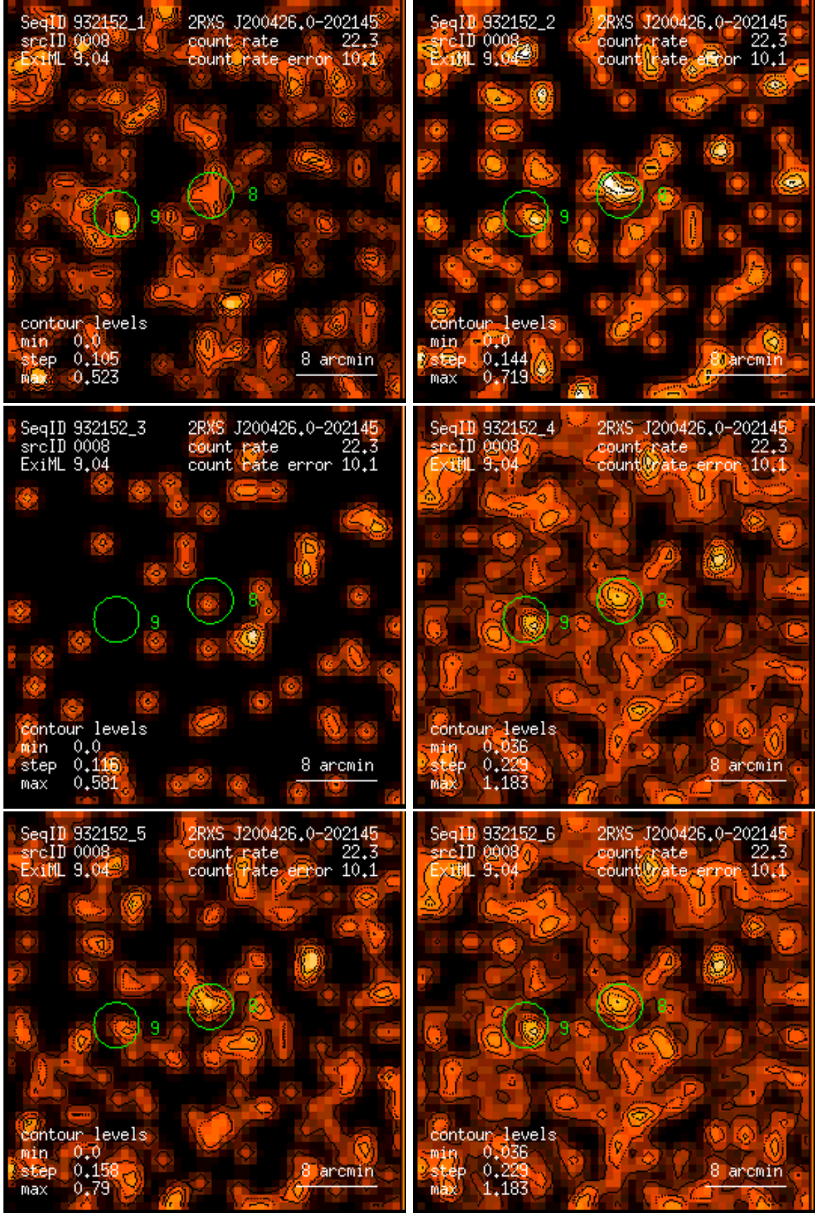
Figure 8: RASS 932152: detection 0008: band rate images, Gaussian filter: (1) PSPC channels 11 – 41, (2) 52 – 90, (3) 91 – 201, (4) 11 – 235, (5) 52 – 201, (6) 11 – 201. Broad band rates in counts/ks. Band rate contour levels in counts/ks/arcmin 2 .
