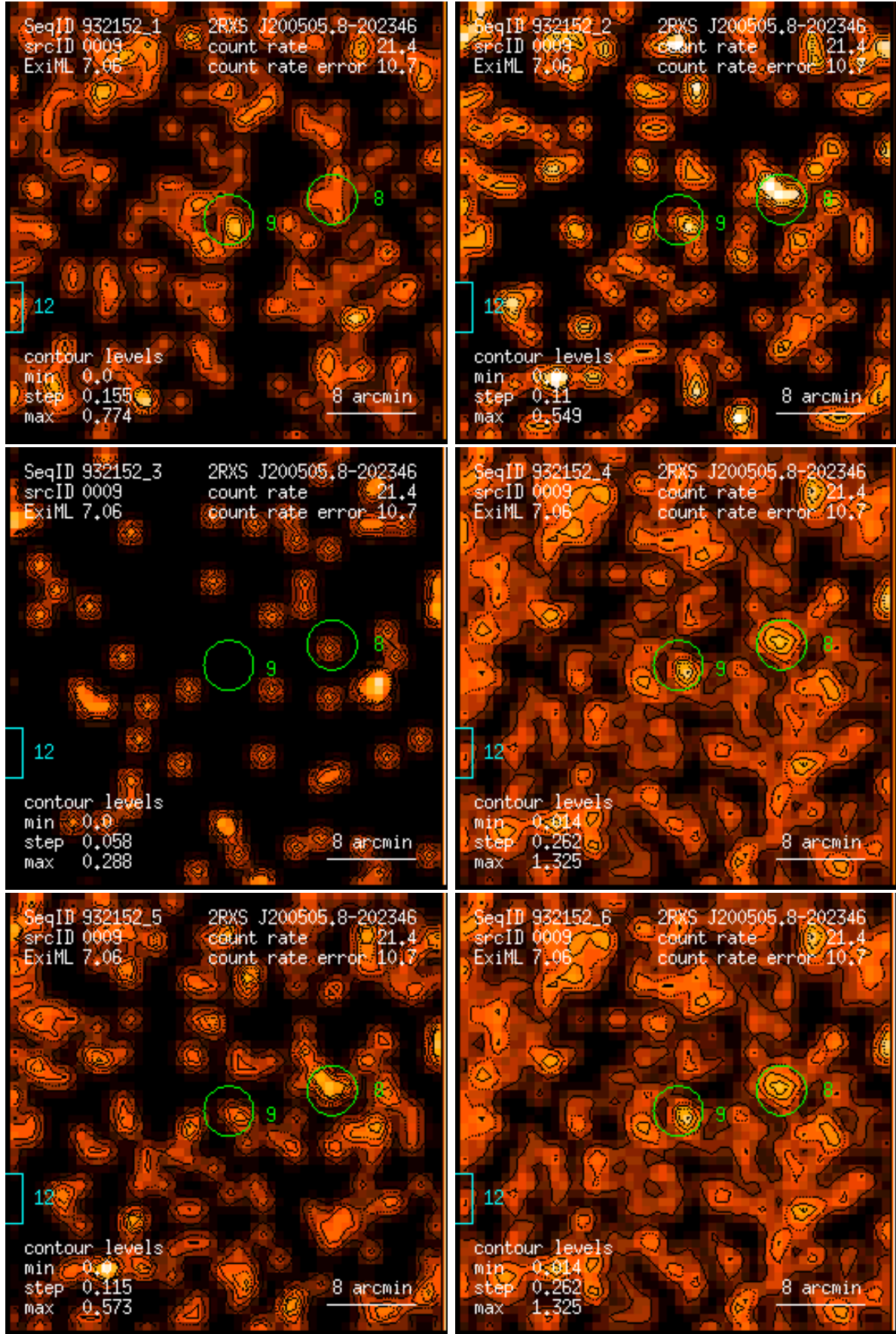
Figure 9: RASS 932152: detection 0009: band rate images, Gaussian filter: (1) PSPC channels 11 – 41, (2) 52 – 90, (3) 91 – 201, (4) 11 – 235, (5) 52 – 201, (6) 11 – 201. Broad band rates in counts/ks. Band rate contour levels in counts/ks/arcmin 2 .
