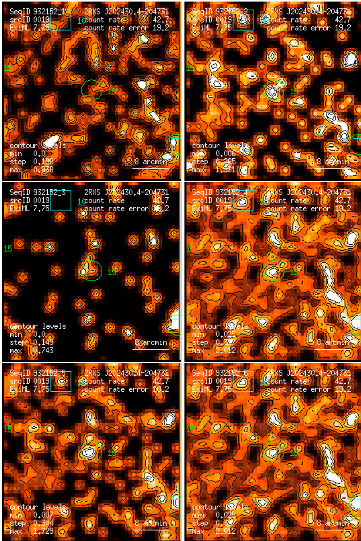
Figure 19: RASS 932152: detection 0019: band rate images, Gaussian filter: (1) PSPC channels 11 – 41, (2) 52 – 90, (3) 91 – 201, (4) 11 – 235, (5) 52 – 201, (6) 11 – 201. Broad band rates in counts/ks. Band rate contour levels in counts/ks/arcmin 2 .
