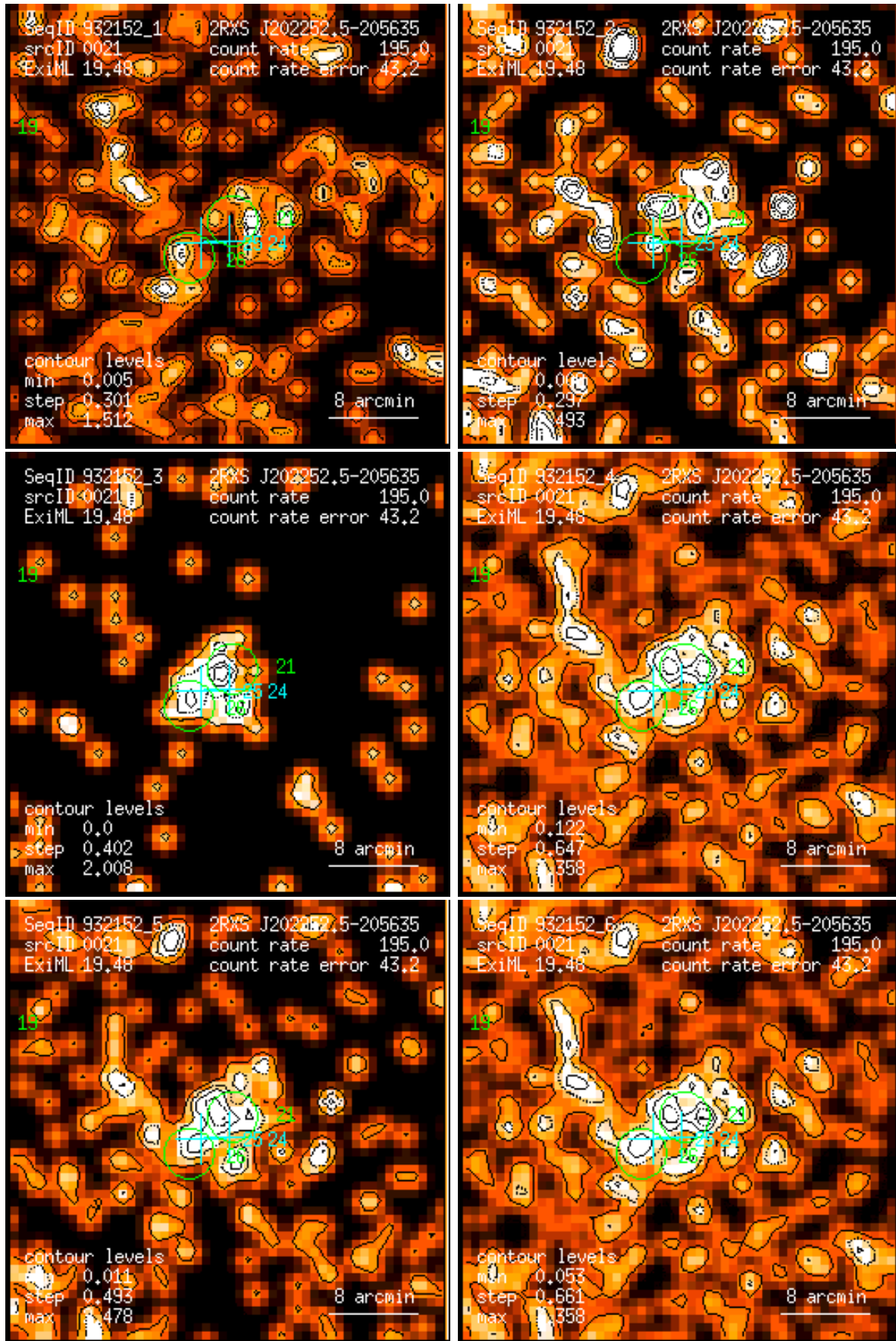
Figure 21: RASS 932152: detection 0021: band rate images, Gaussian filter: (1) PSPC channels 11 – 41, (2) 52 – 90, (3) 91 – 201, (4) 11 – 235, (5) 52 – 201, (6) 11 – 201. Broad band rates in counts/ks. Band rate contour levels in counts/ks/arcmin 2 .
