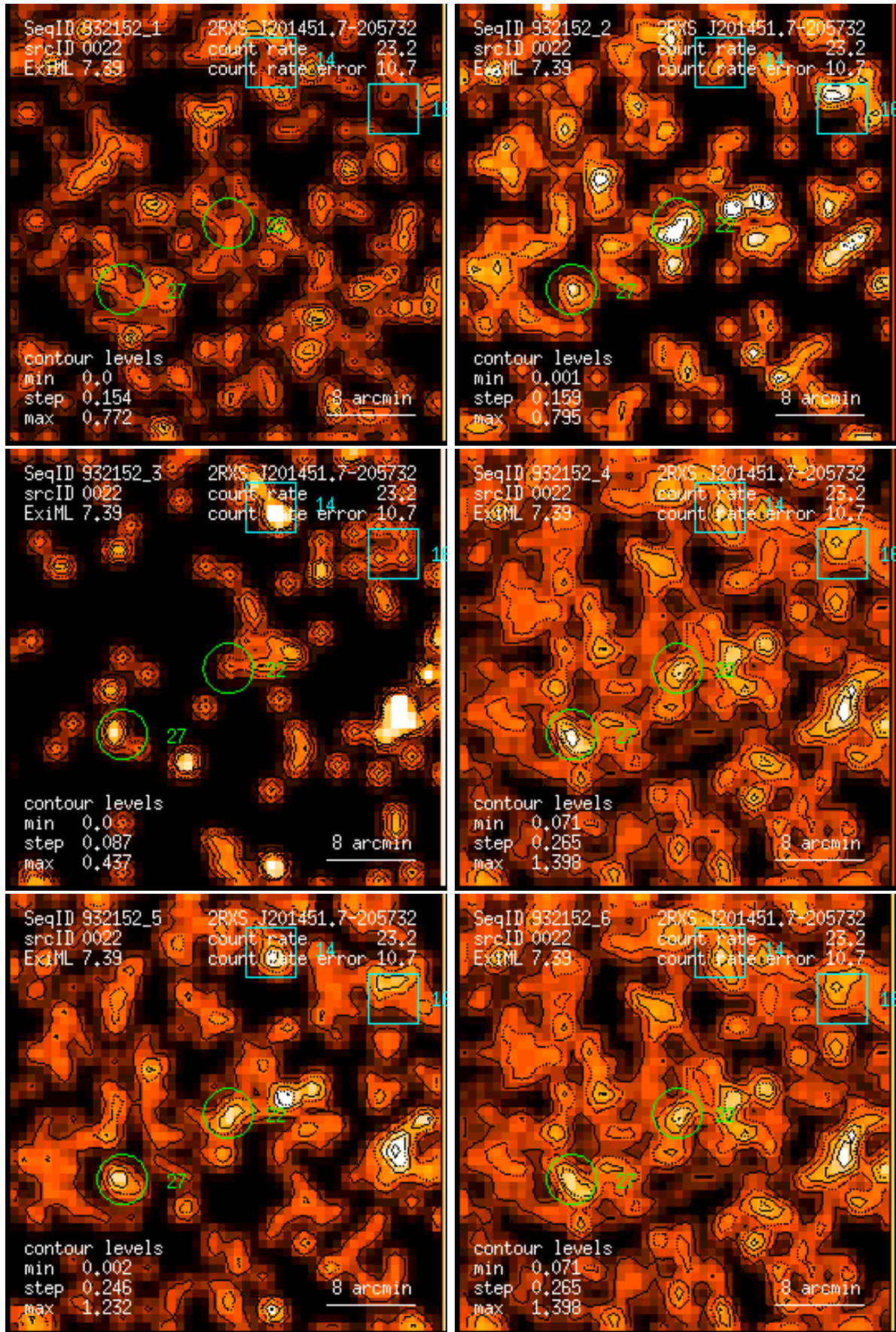
Figure 22: RASS 932152: detection 0022: band rate images, Gaussian filter: (1) PSPC channels 11 – 41, (2) 52 – 90, (3) 91 – 201, (4) 11 – 235, (5) 52 – 201, (6) 11 – 201. Broad band rates in counts/ks. Band rate contour levels in counts/ks/arcmin 2 .
