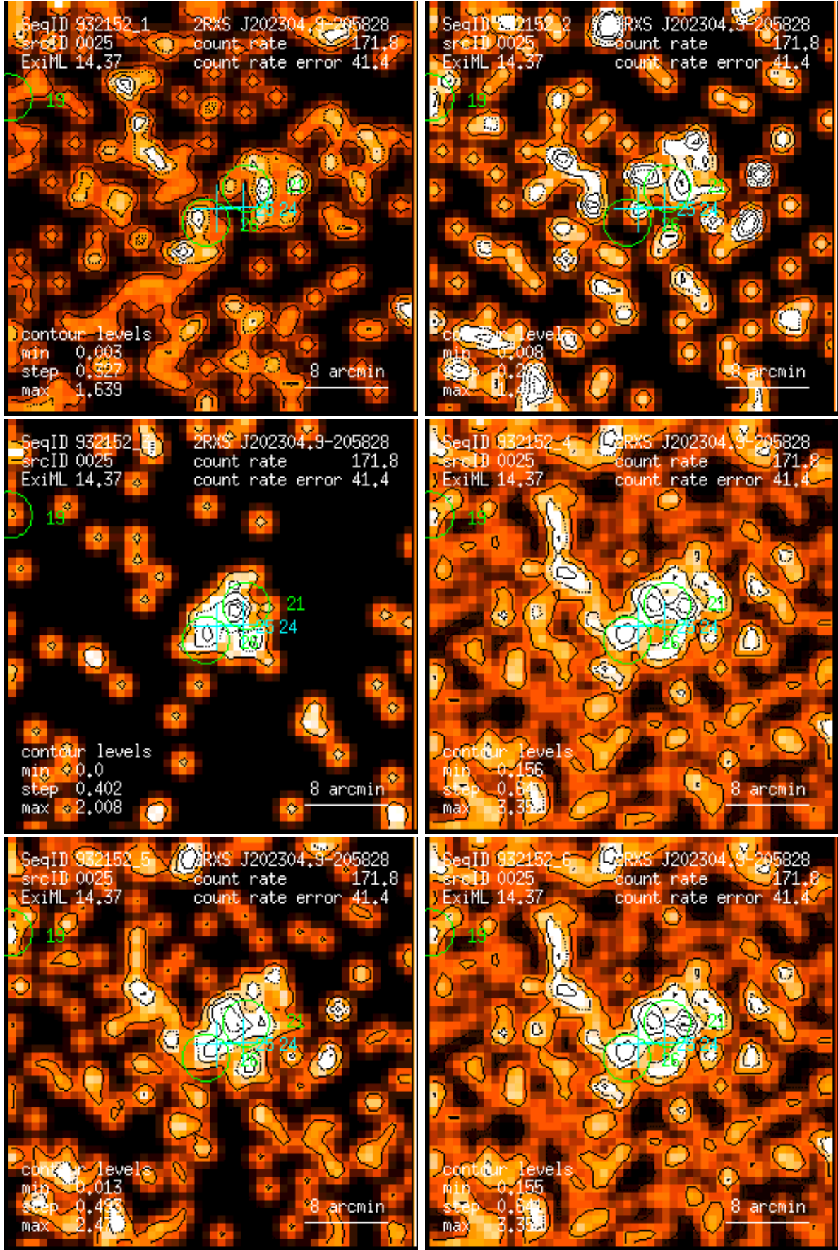
Figure 25: RASS 932152: detection 0025: band rate images, Gaussian filter: (1) PSPC channels 11 – 41, (2) 52 – 90, (3) 91 – 201, (4) 11 – 235, (5) 52 – 201, (6) 11 – 201. Broad band rates in counts/ks. Band rate contour levels in counts/ks/arcmin 2 .
