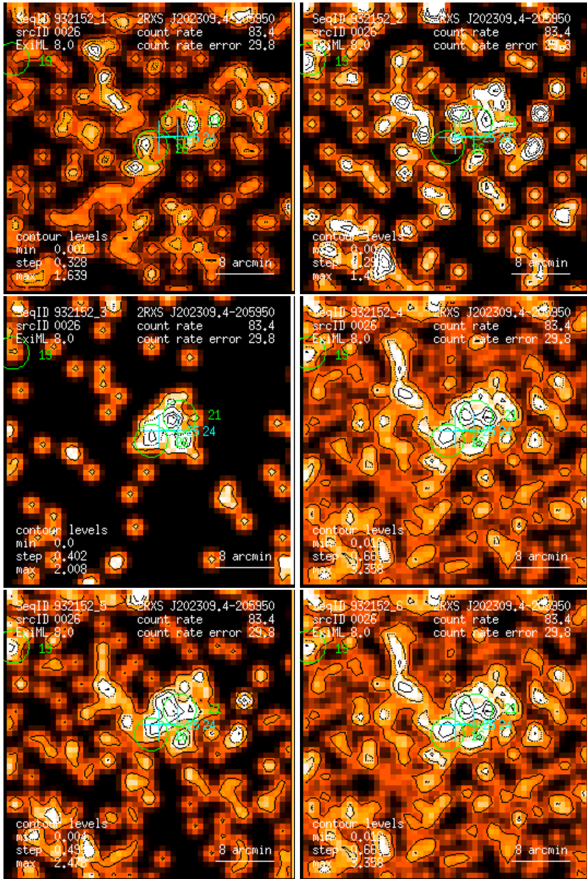
Figure 26: RASS 932152: detection 0026: band rate images, Gaussian filter: (1) PSPC channels 11 – 41, (2) 52 – 90, (3) 91 – 201, (4) 11 – 235, (5) 52 – 201, (6) 11 – 201. Broad band rates in counts/ks. Band rate contour levels in counts/ks/arcmin 2 .
