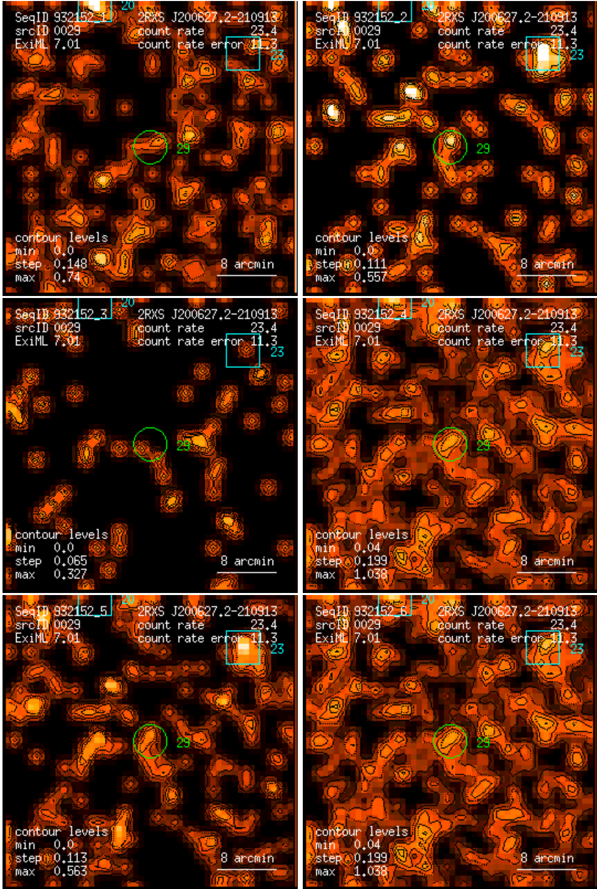
Figure 29: RASS 932152: detection 0029: band rate images, Gaussian filter: (1) PSPC channels 11 – 41, (2) 52 – 90, (3) 91 – 201, (4) 11 – 235, (5) 52 – 201, (6) 11 – 201. Broad band rates in counts/ks. Band rate contour levels in counts/ks/arcmin 2 .
