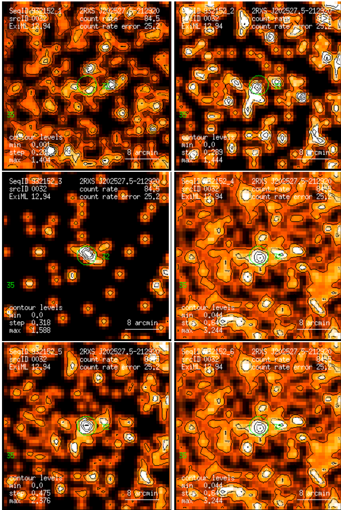
Figure 32: RASS 932152: detection 0032: band rate images, Gaussian filter: (1) PSPC channels 11 – 41, (2) 52 – 90, (3) 91 – 201, (4) 11 – 235, (5) 52 – 201, (6) 11 – 201. Broad band rates in counts/ks. Band rate contour levels in counts/ks/arcmin 2 .
