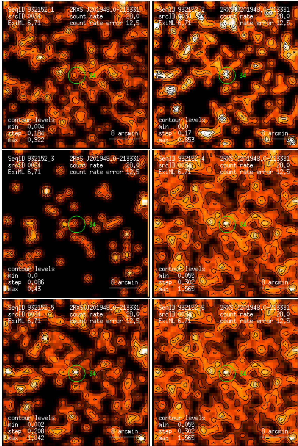
Figure 34: RASS 932152: detection 0034: band rate images, Gaussian filter: (1) PSPC channels 11 – 41, (2) 52 – 90, (3) 91 – 201, (4) 11 – 235, (5) 52 – 201, (6) 11 – 201. Broad band rates in counts/ks. Band rate contour levels in counts/ks/arcmin 2 .
