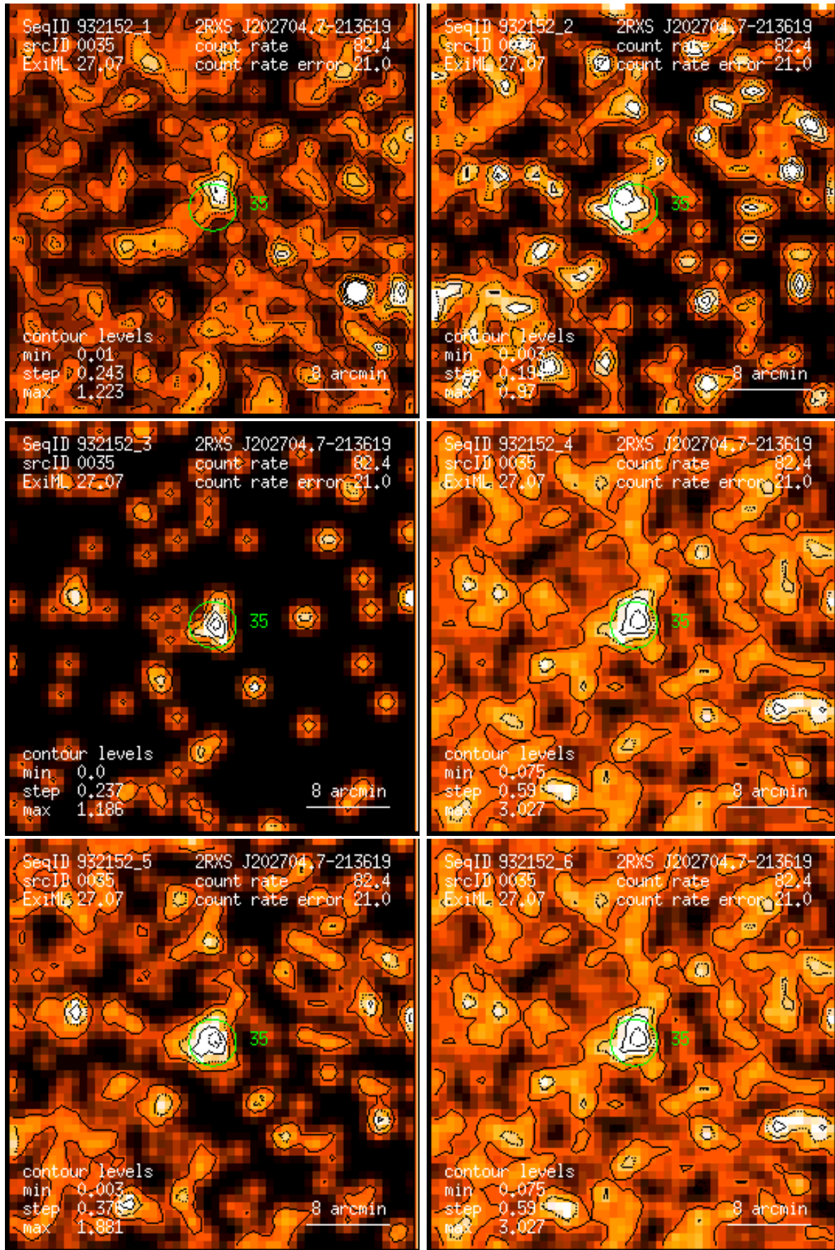
Figure 35: RASS 932152: detection 0035: band rate images, Gaussian filter: (1) PSPC channels 11 – 41, (2) 52 – 90, (3) 91 – 201, (4) 11 – 235, (5) 52 – 201, (6) 11 – 201. Broad band rates in counts/ks. Band rate contour levels in counts/ks/arcmin 2 .
