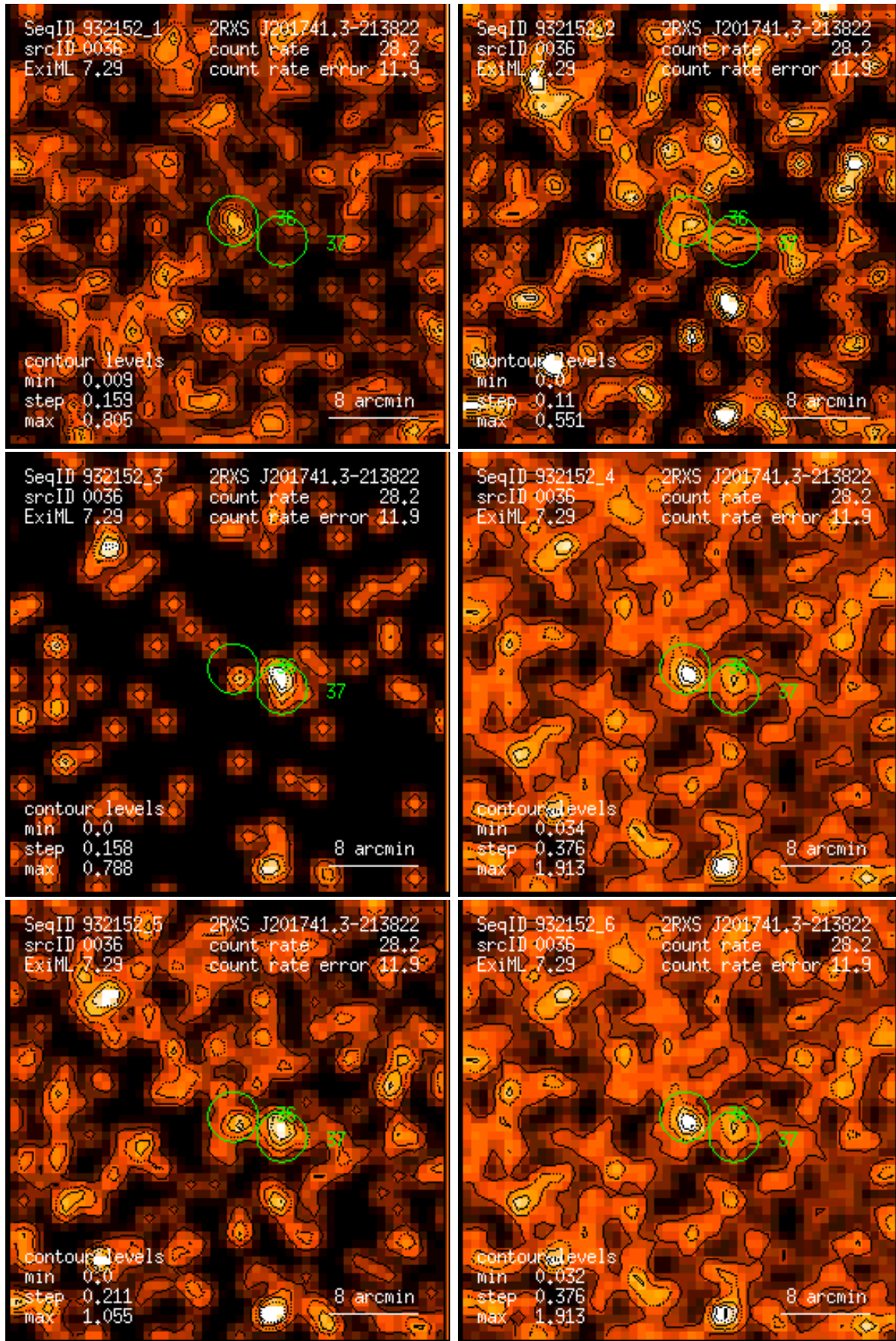
Figure 36: RASS 932152: detection 0036: band rate images, Gaussian filter: (1) PSPC channels 11 – 41, (2) 52 – 90, (3) 91 – 201, (4) 11 – 235, (5) 52 – 201, (6) 11 – 201. Broad band rates in counts/ks. Band rate contour levels in counts/ks/arcmin 2 .
