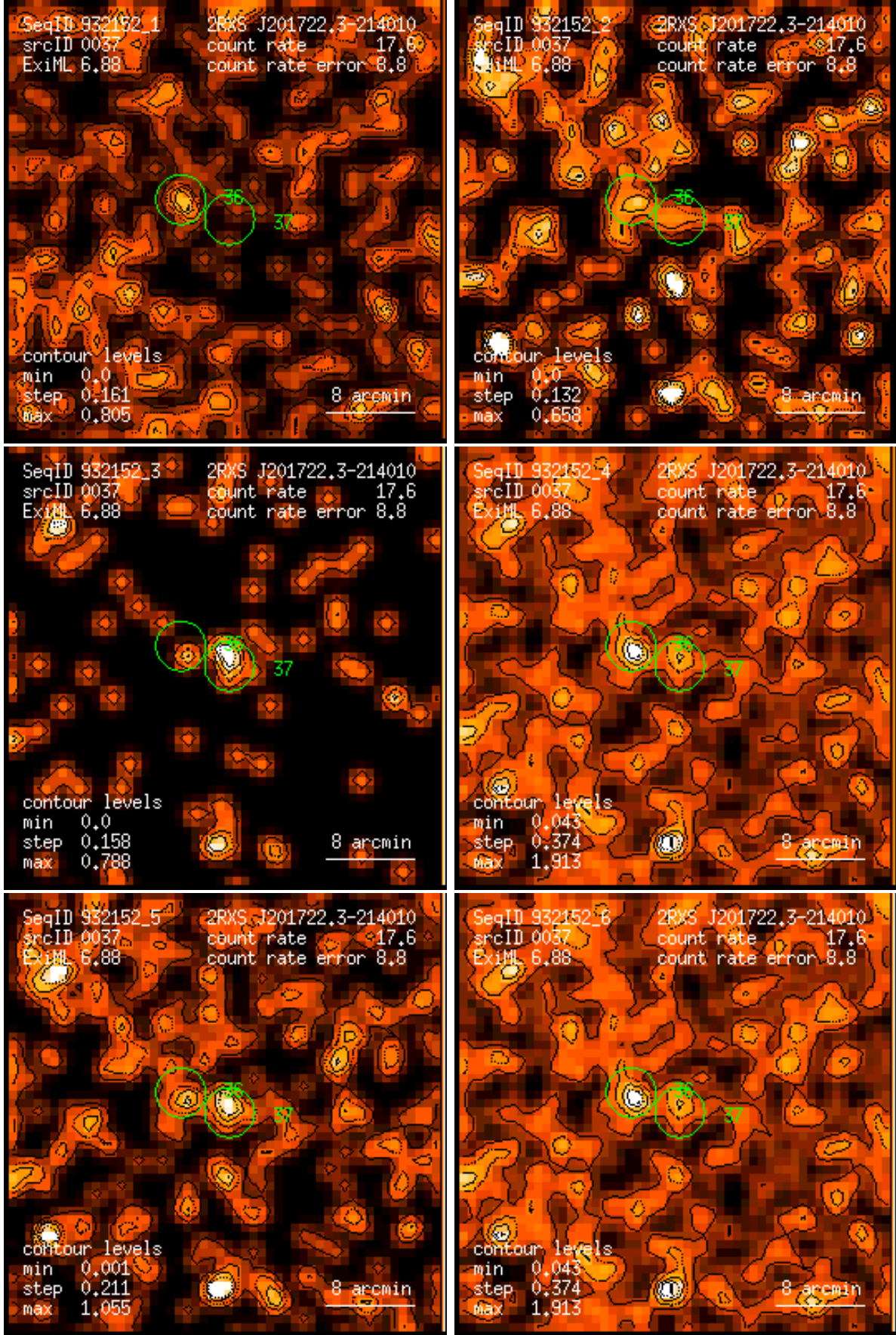
Figure 37: RASS 932152: detection 0037: band rate images, Gaussian filter: (1) PSPC channels 11 – 41, (2) 52 – 90, (3) 91 – 201, (4) 11 – 235, (5) 52 – 201, (6) 11 – 201. Broad band rates in counts/ks. Band rate contour levels in counts/ks/arcmin 2 .
