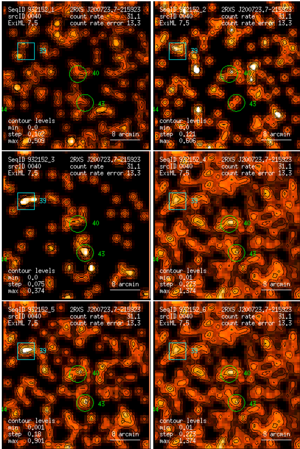
Figure 40: RASS 932152: detection 0040: band rate images, Gaussian filter: (1) PSPC channels 11 – 41, (2) 52 – 90, (3) 91 – 201, (4) 11 – 235, (5) 52 – 201, (6) 11 – 201. Broad band rates in counts/ks. Band rate contour levels in counts/ks/arcmin 2 .
