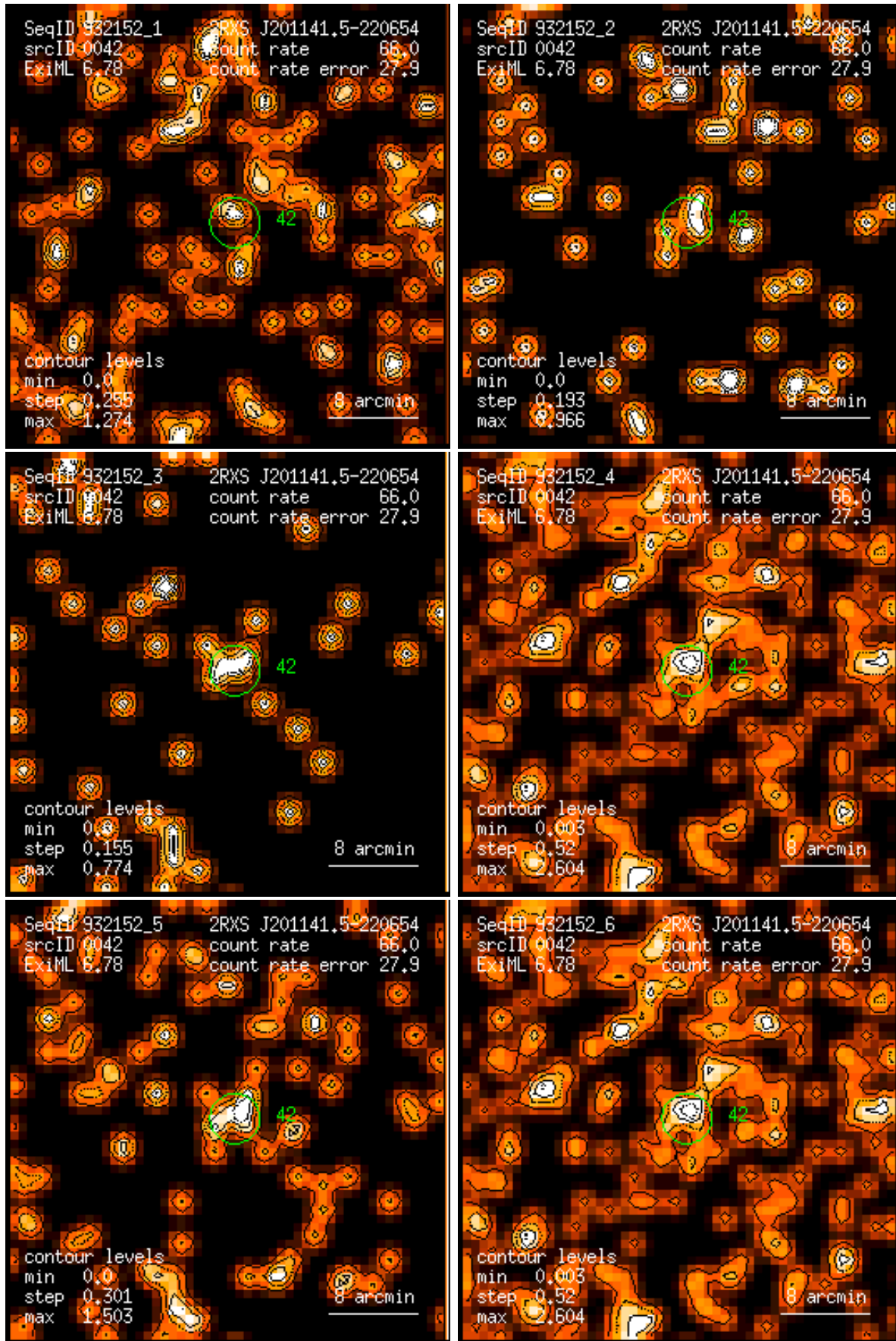
Figure 42: RASS 932152: detection 0042: band rate images, Gaussian filter: (1) PSPC channels 11 – 41, (2) 52 – 90, (3) 91 – 201, (4) 11 – 235, (5) 52 – 201, (6) 11 – 201. Broad band rates in counts/ks. Band rate contour levels in counts/ks/arcmin 2 .
