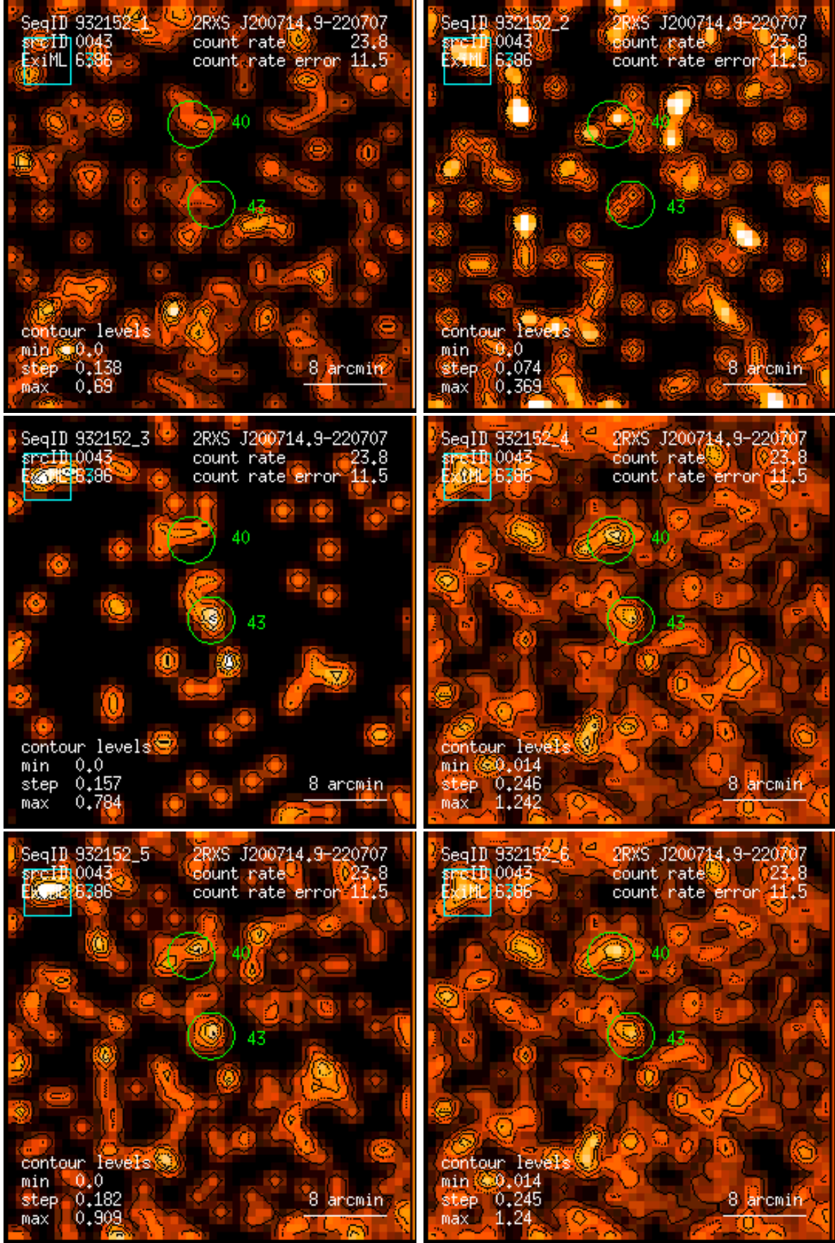
Figure 43: RASS 932152: detection 0043: band rate images, Gaussian filter: (1) PSPC channels 11 – 41, (2) 52 – 90, (3) 91 – 201, (4) 11 – 235, (5) 52 – 201, (6) 11 – 201. Broad band rates in counts/ks. Band rate contour levels in counts/ks/arcmin 2 .
