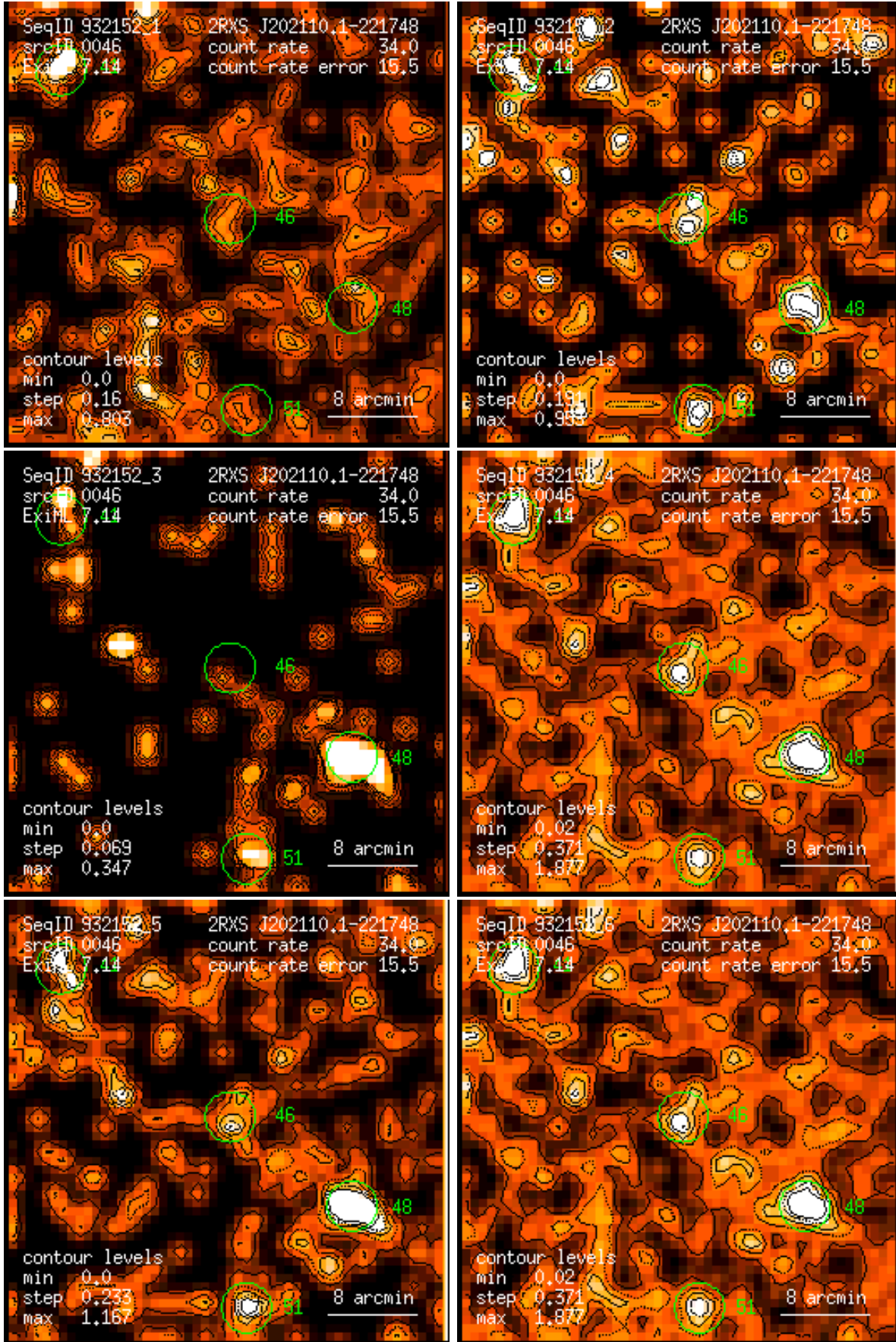
Figure 46: RASS 932152: detection 0046: band rate images, Gaussian filter: (1) PSPC channels 11 – 41, (2) 52 – 90, (3) 91 – 201, (4) 11 – 235, (5) 52 – 201, (6) 11 – 201. Broad band rates in counts/ks. Band rate contour levels in counts/ks/arcmin 2 .
